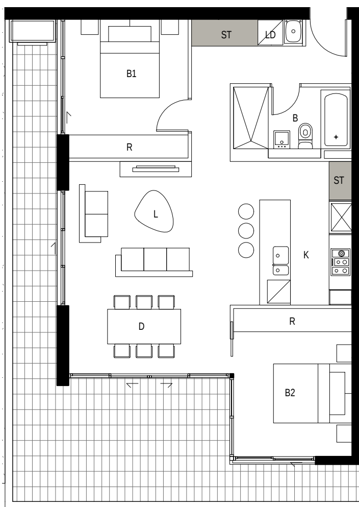
7 DETAIL PLAN BLDG A - Apartment Type 5 2 BED - 74sqm Storage - 4.8cm
