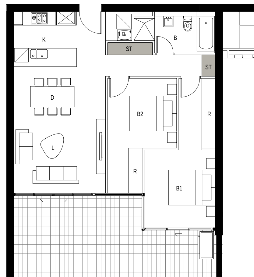
8 DETAIL PLAN BLDG A - Apartment Type 6 2 BED - 77sqm Storage 6.3cm
