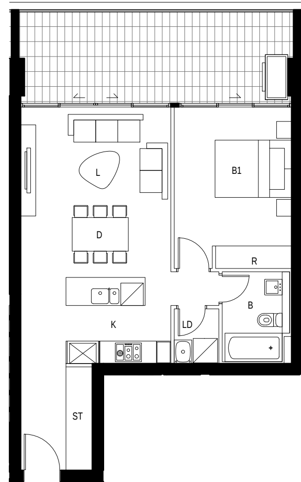
12 DETAIL PLAN BLDG A - Apartment Type 12 1 BED - 55sqm Storage - 5cm
