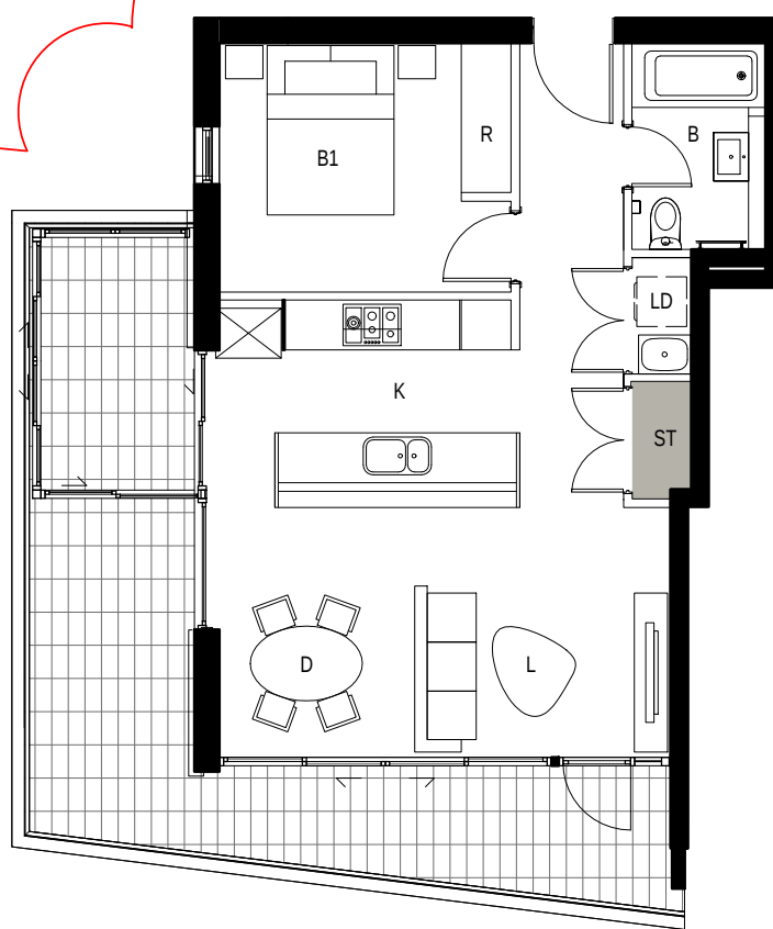
11 DETAIL PLAN BLDG A - Apartment Type 13 1 BED - 55sqm Storage - 5cm
