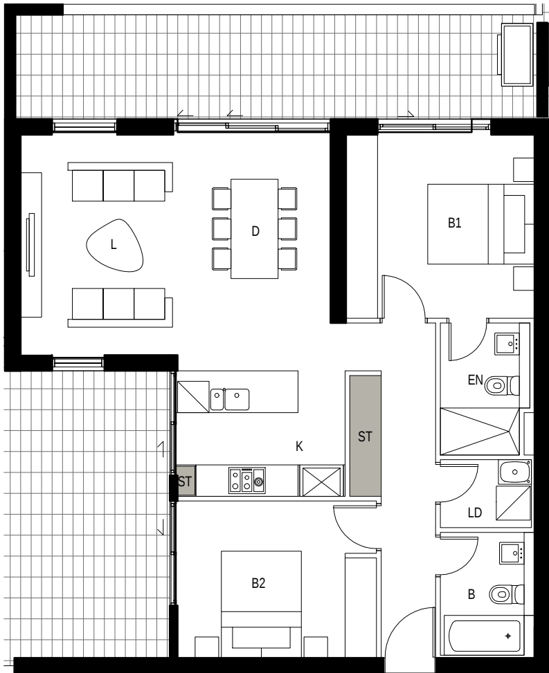
5 DETAIL PLAN BLDG A - Apartment Type 1 2 BED - 80sqm Storage - 2cm
