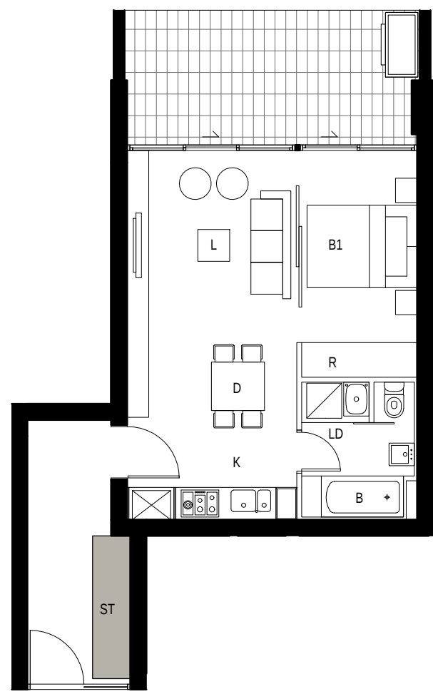
2 DETAIL PLAN BLDG A - Apartment Type 3 1 BED - 55sqm Storage - 5cm
