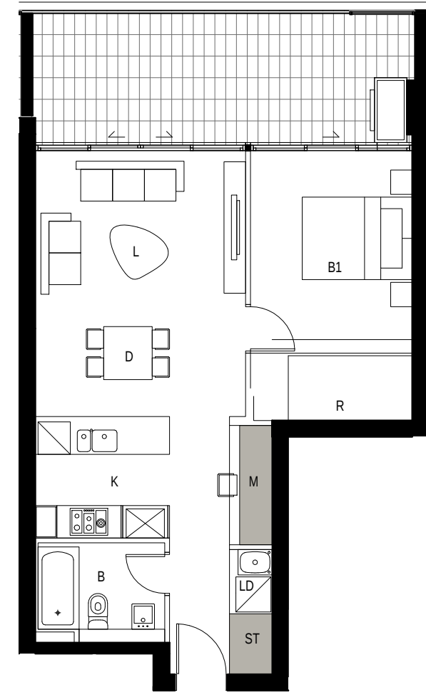
1 DETAIL PLAN BLDG A - Apartment Type 2 1 BED - 55sqm Storage - 3cm(Includes Media Room)
