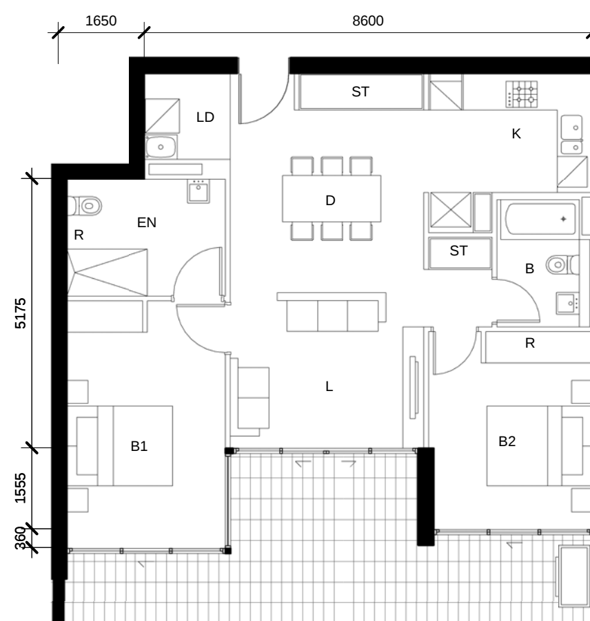
3 DETAIL PLAN BLDG A - Apartment Type 7-A Pre Adaption Layout
