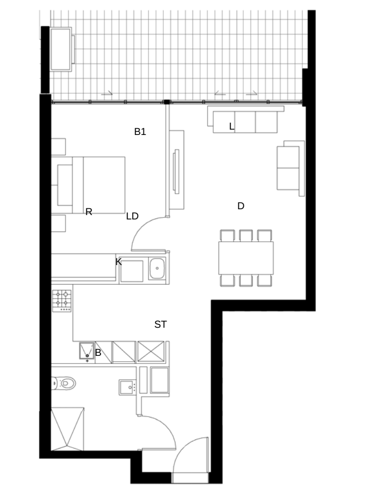
1 DETAIL PLAN BLDG A - Apartment Type 2-A Pre Adaption Layout
