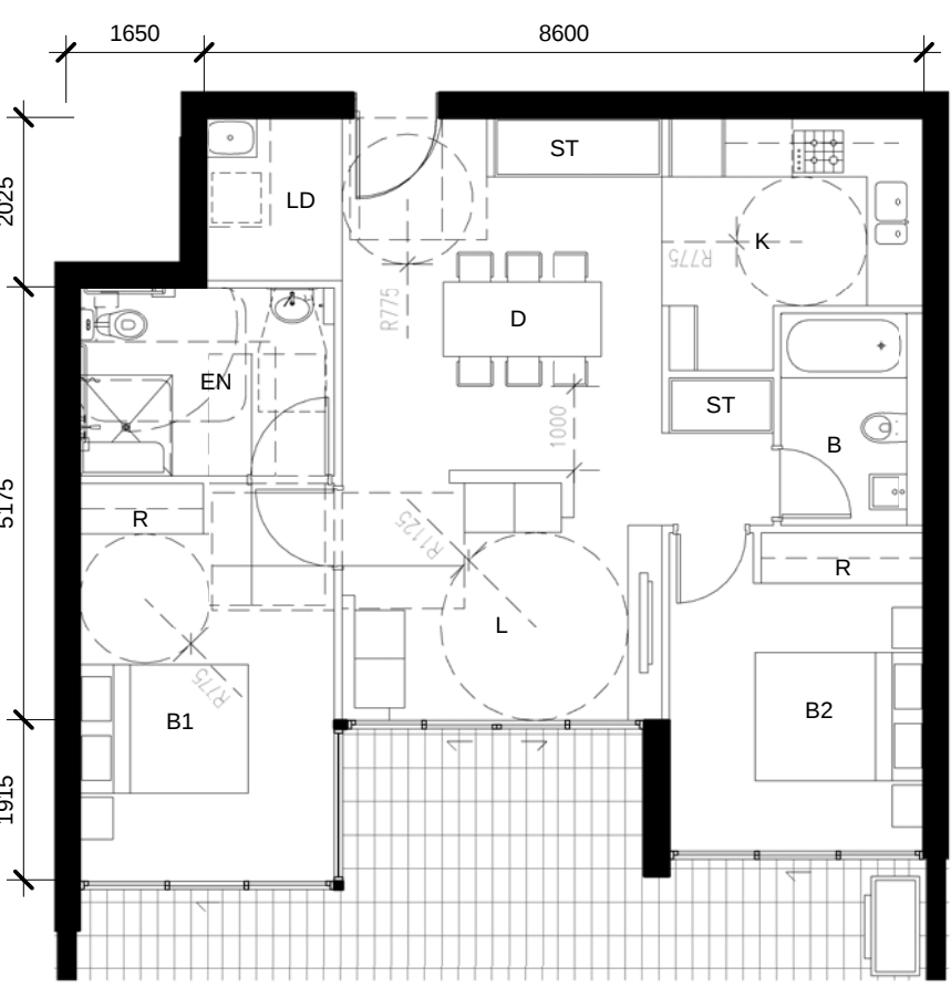
4 DETAIL PLAN BLDG A - Apartment Type 7-A Post Adaption Layout
