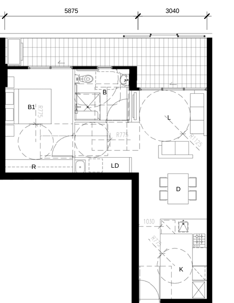
10 DETAIL PLAN BLDG D - Apartment Type 12-A Post Adaption Layout
