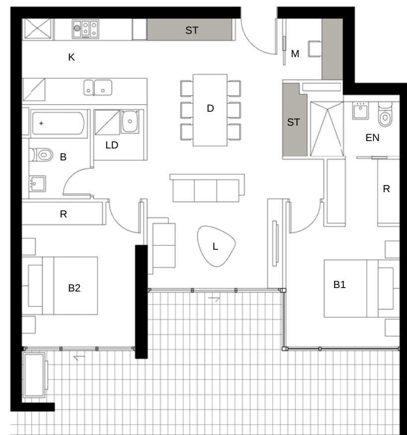
6 DETAIL PLAN BLDG D - Apartment Type 6 2 BED - 79sqm Storage - 7cbm(Includes Media Room)
