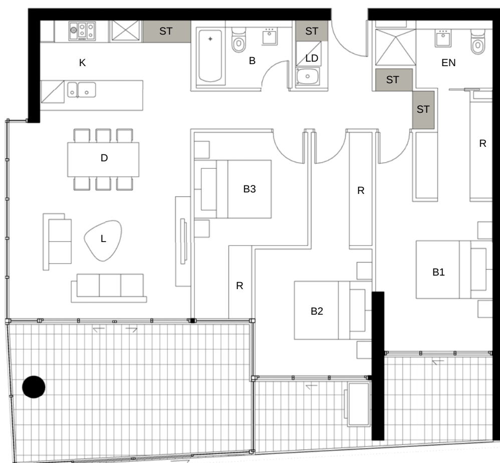
10 DETAIL PLAN BLDG D - Apartment Type 10 3 BED - 106sqm Storage - 5cbm
