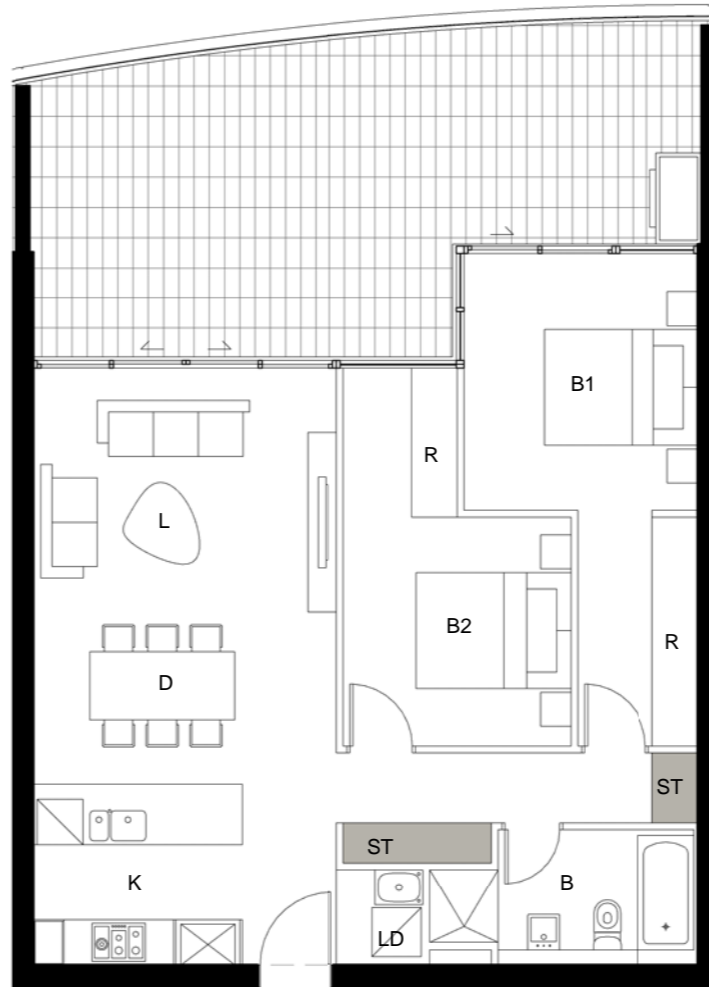
7 DETAIL PLAN BLDG C - Apartment Type 2 2 BED - 74sqm Storage - 4cbm
