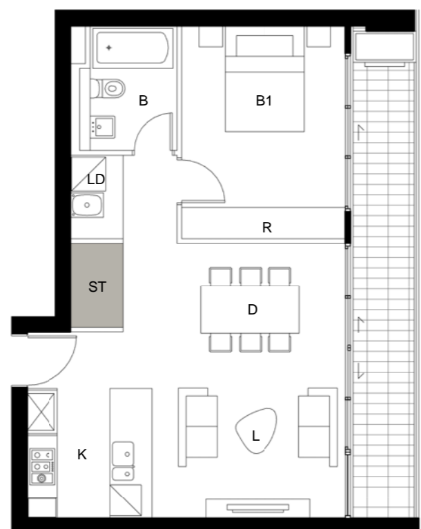
5 DETAIL PLAN BLDG C - Apartment Type 4 1 BED - 53sqm Storage - 3.5cbm
