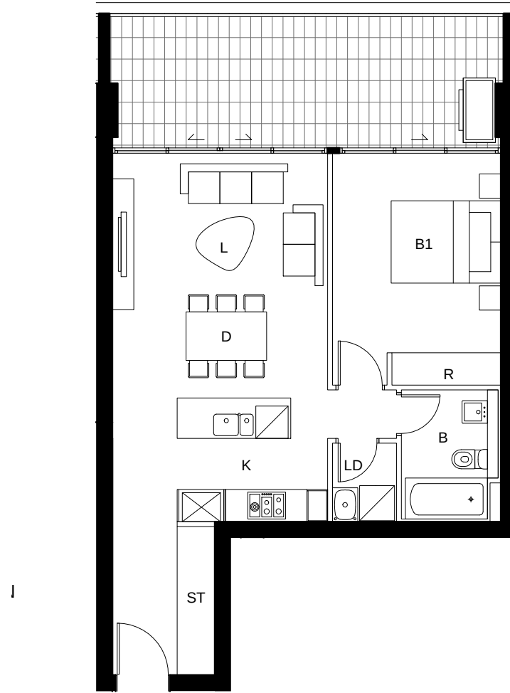
12 DETAIL PLAN BLDG A - Apartment Type 12 1 BED - 55sqm Storage - 5cbm
