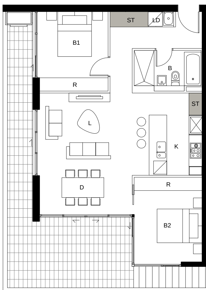
7 DETAIL PLAN BLDG A - Apartment Type 5 2 BED - 74sqm Storage - 4.8cbm
