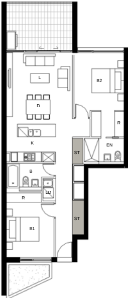
4 DETAIL PLAN BLDG D - Apartment Type 4 2 BED - 79sqm Storage 6.3cbm
