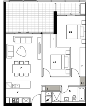
15 DETAIL PLAN BLDG E - Apartment Type 1 2 BED - 71sqm Storage - 4cbm
