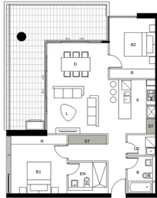
8 DETAIL PLAN BLDG D - Apartment Type 8 2 BED - 84sqm Storage - 4cbm
