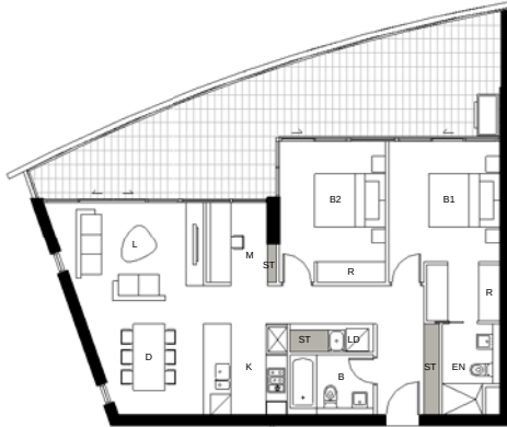
6 DETAIL PLAN BLDG C - Apartment Type 1 2 BED - 85sqm Storage - 4cbm
