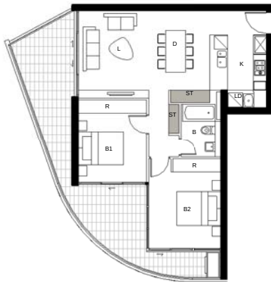
8 DETAIL PLAN BLDG C - Apartment Type 3 2 BED - 70sqm Storage - 4cbm
