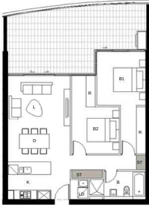
7 DETAIL PLAN BLDG C - Apartment Type 2 2 BED - 74sqm Storage - 4cbm
