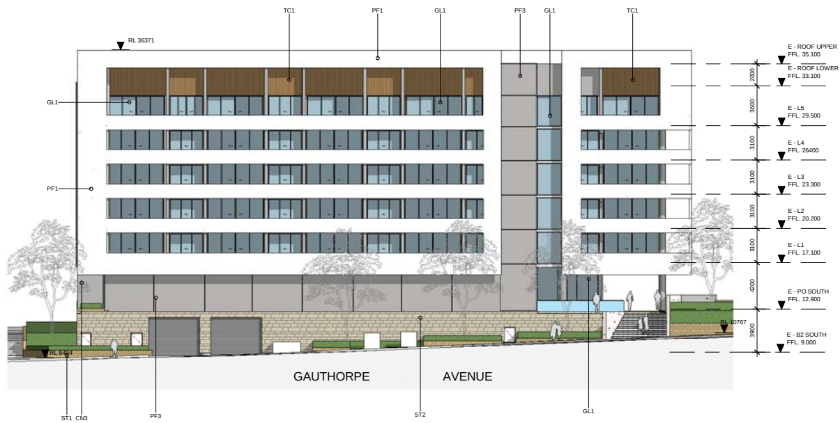
2 ELEVATION BLDG E - SOUTH 1 : 200
