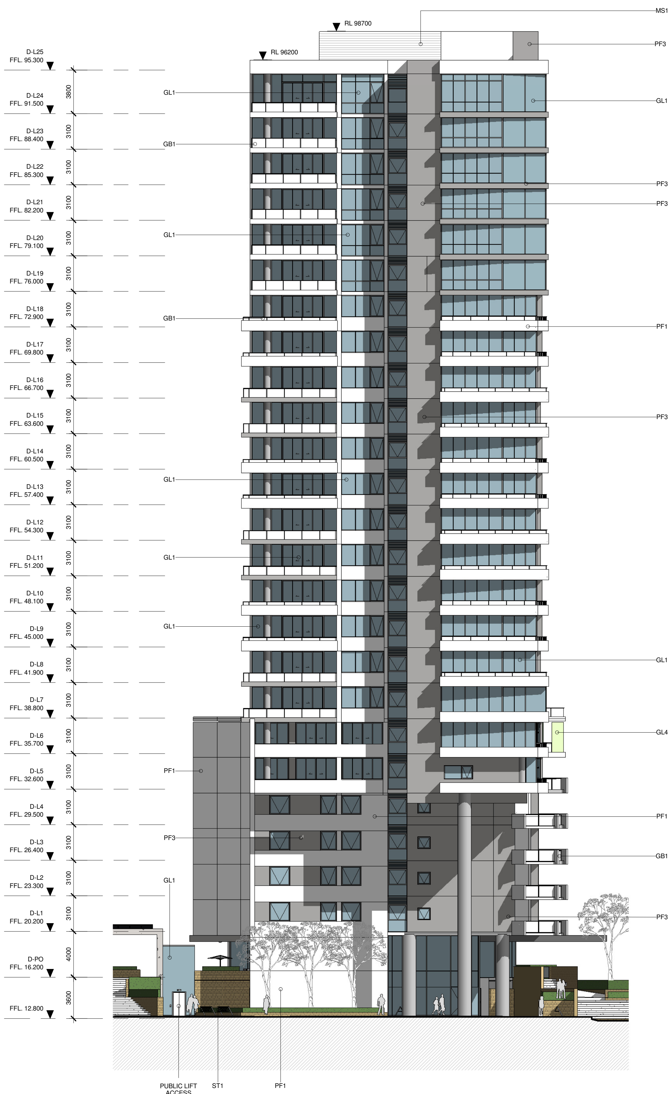
1 ELEVATION BLDG D - SOUTH 1 : 200
