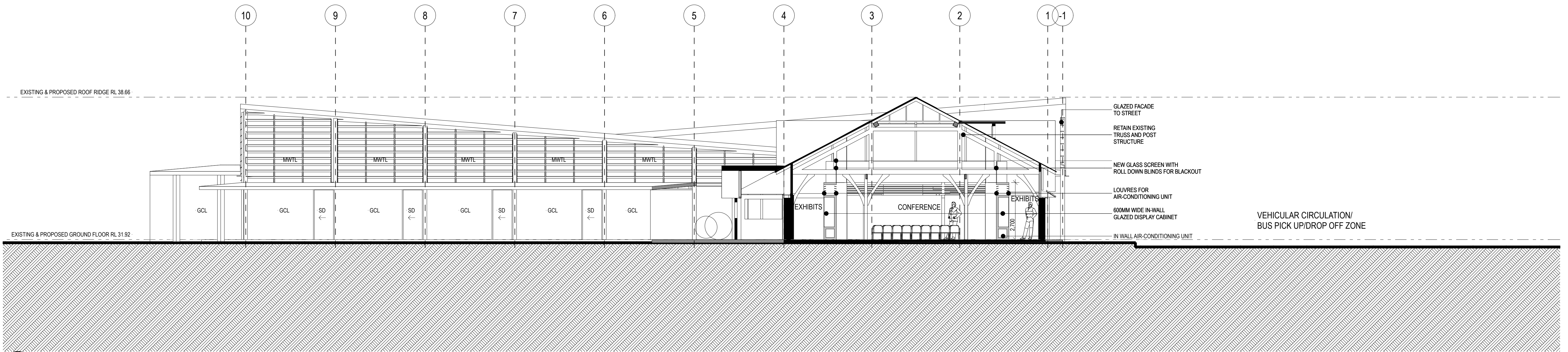
1 CROSS SECTION 1:100
