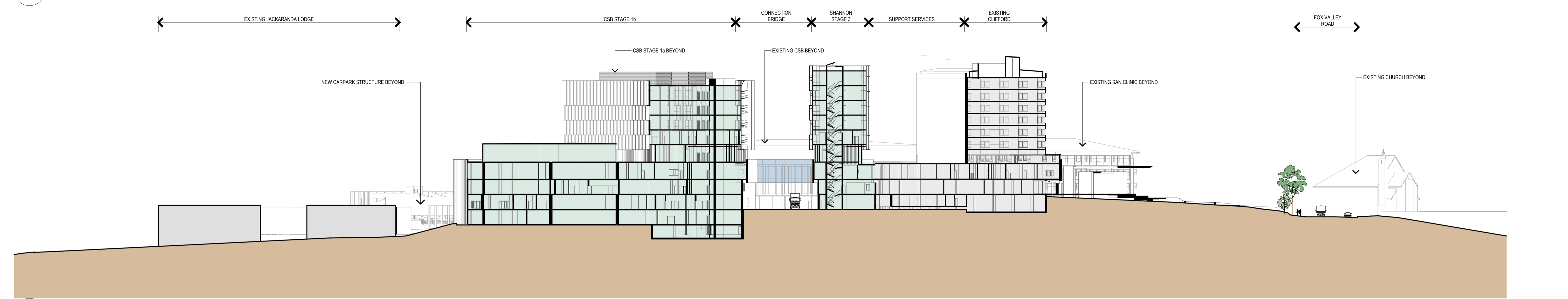
02 Site Sections East-West SCALE 1:500
