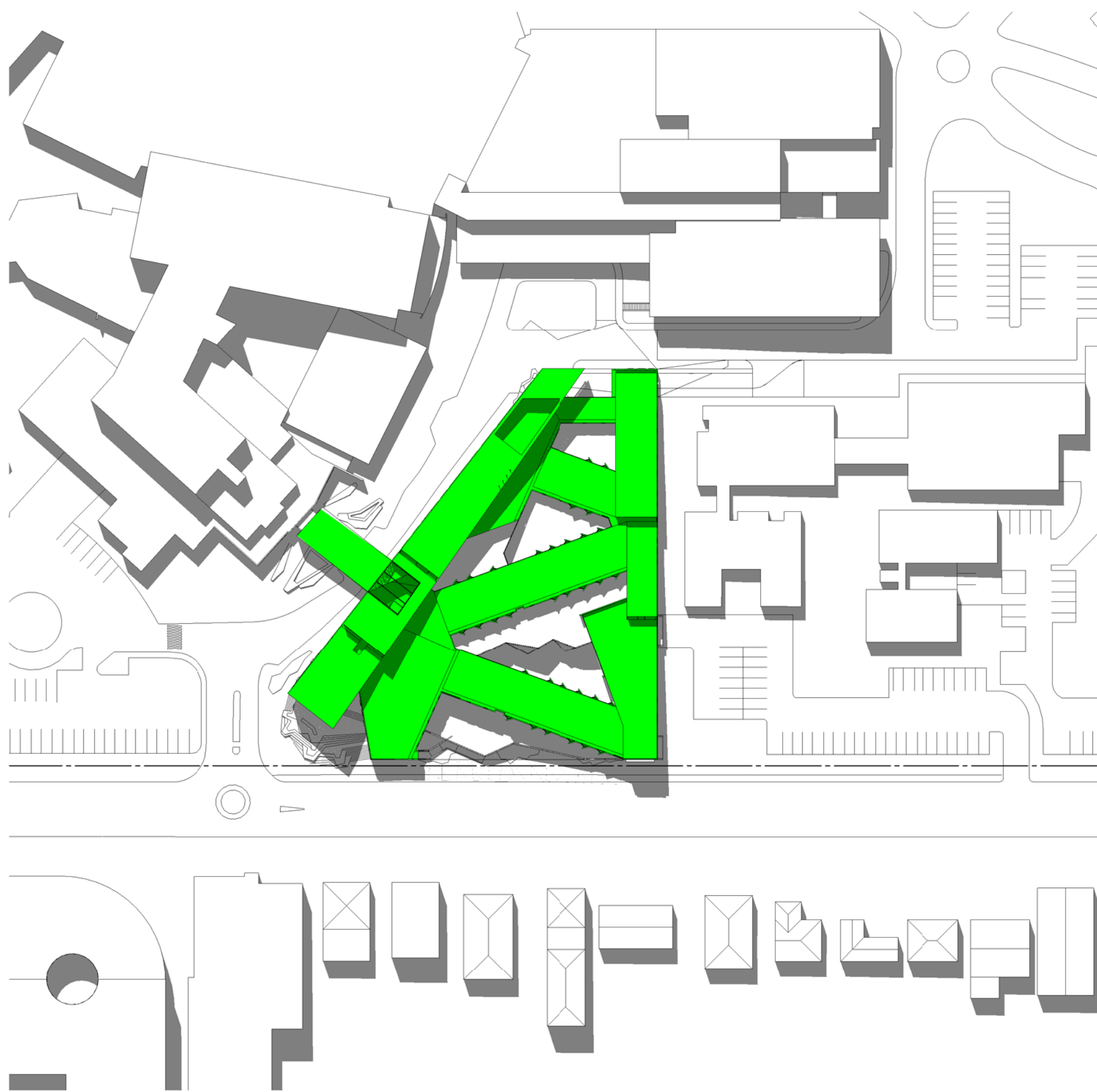
2 PROPOSED SHADOW DIAGRAM - SEPTEMBER 12PM 1 : 1000
