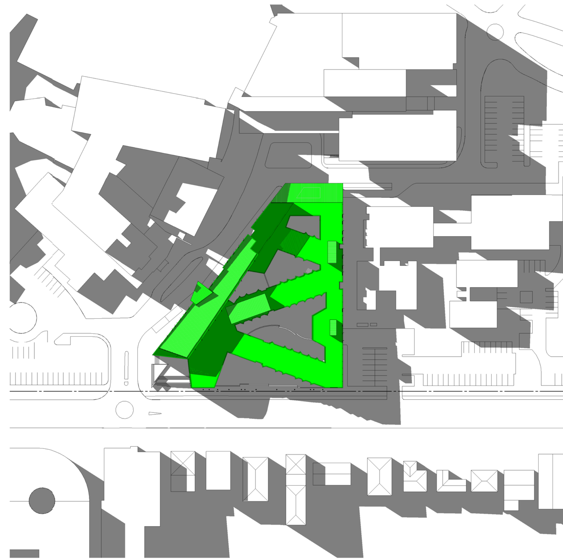
3 PROPOSED SHADOW DIAGRAM - JUNE 3PM 1 : 1000
