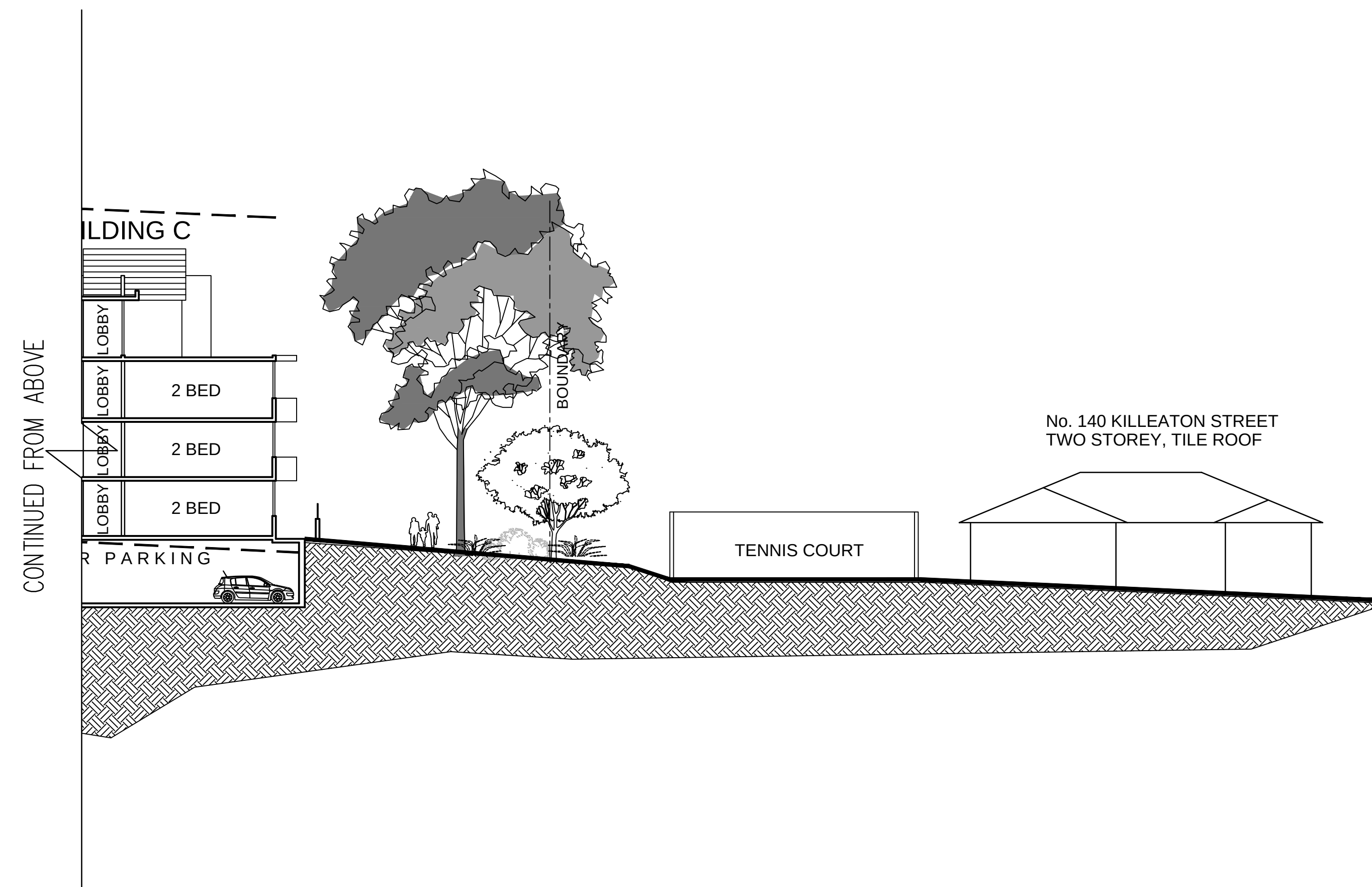
SITE SECTION B-B SCALE 1:200
