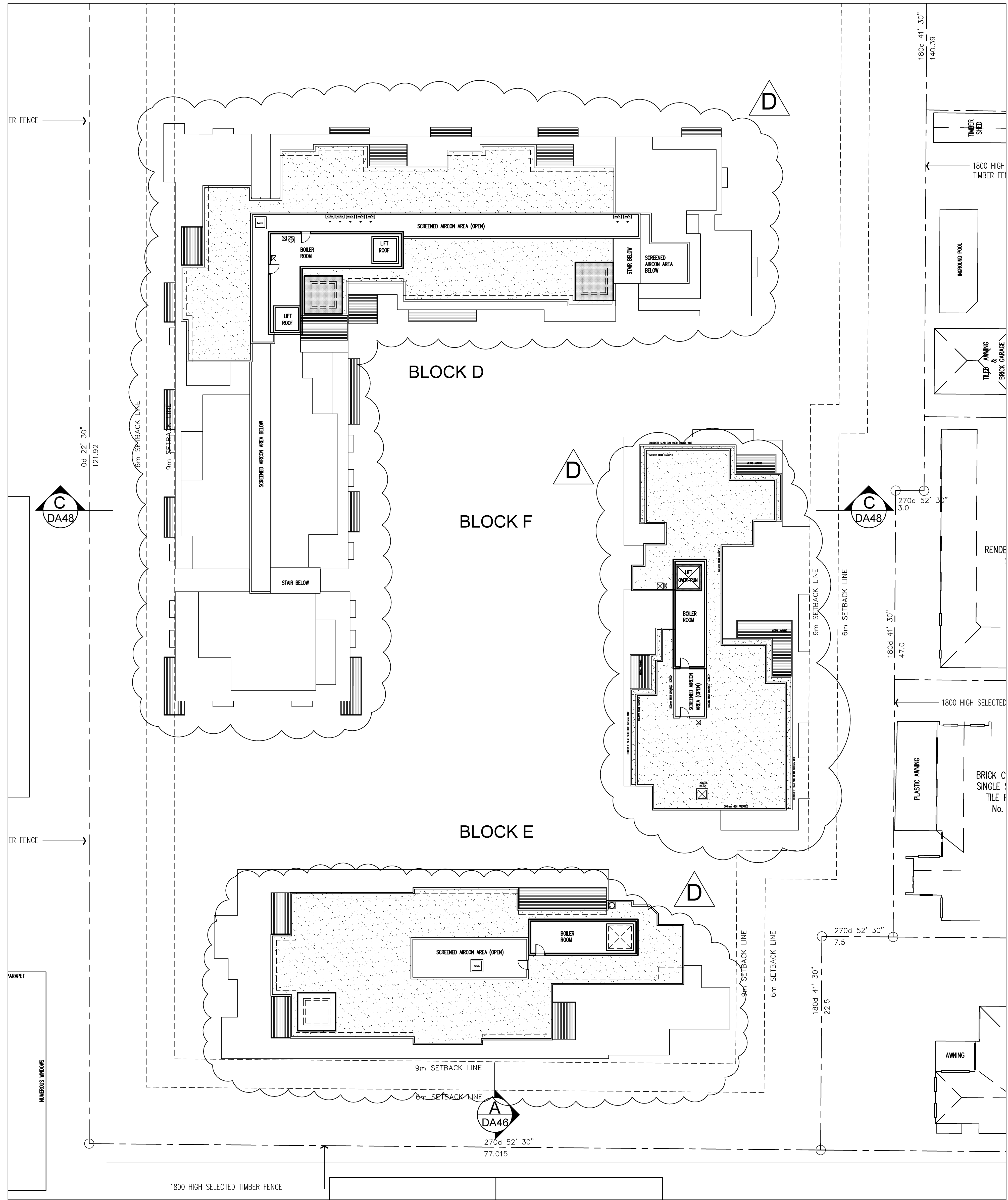
STAGE-1 LEVEL ROOF PLAN
