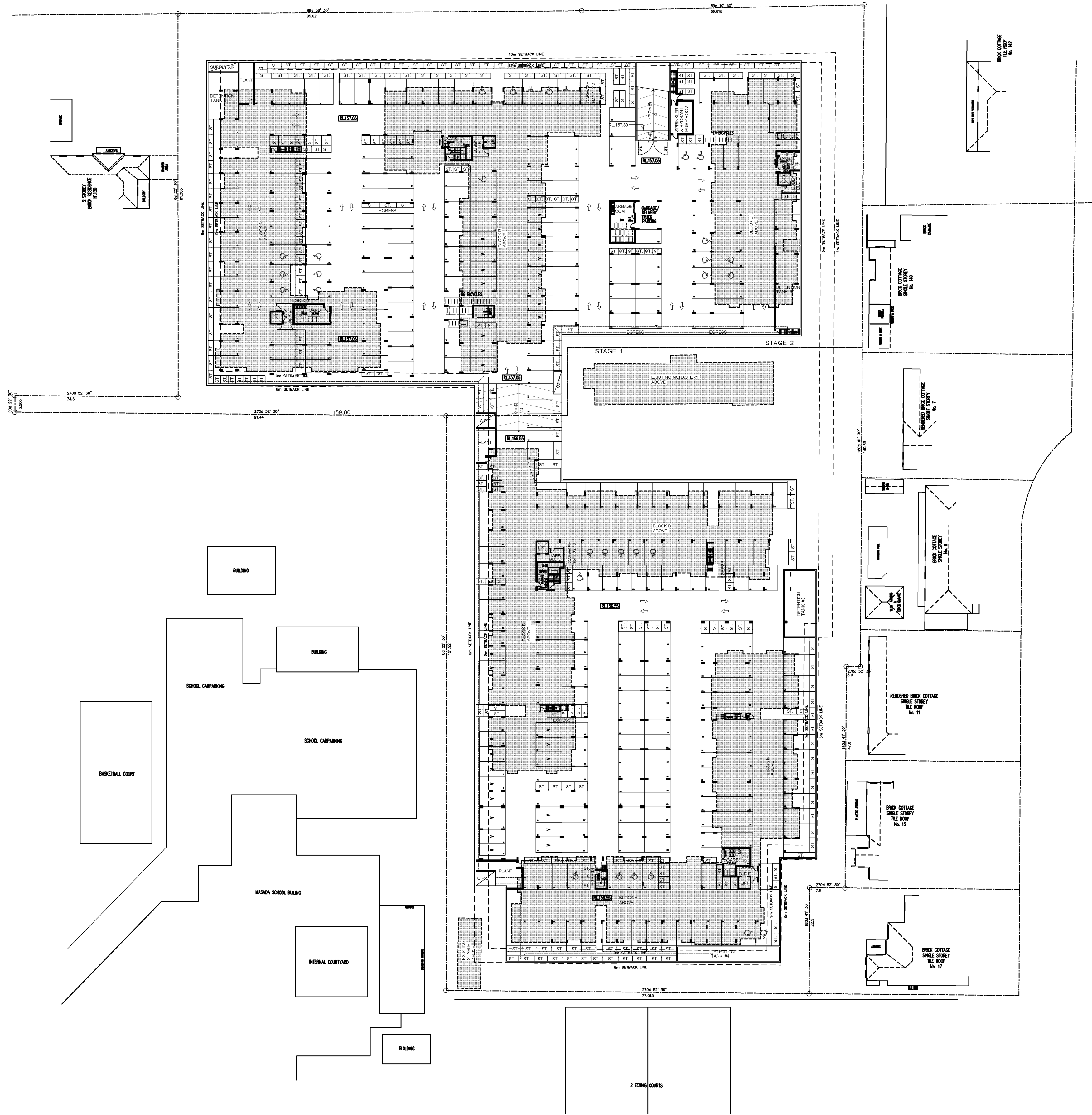
CARPARK PLAN SCALE 1:500
