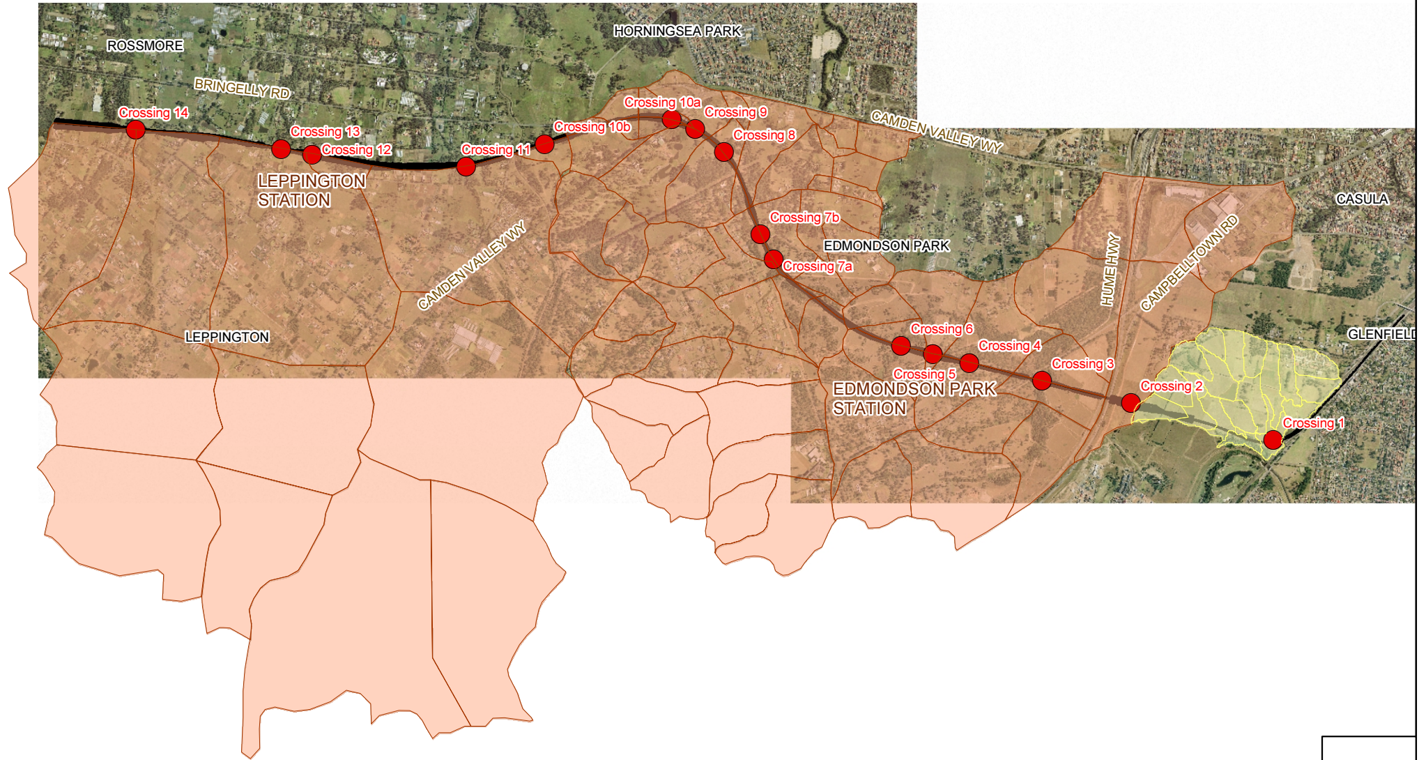
FIGURE 2 HYDROLOGIC MODEL LAYOUT
