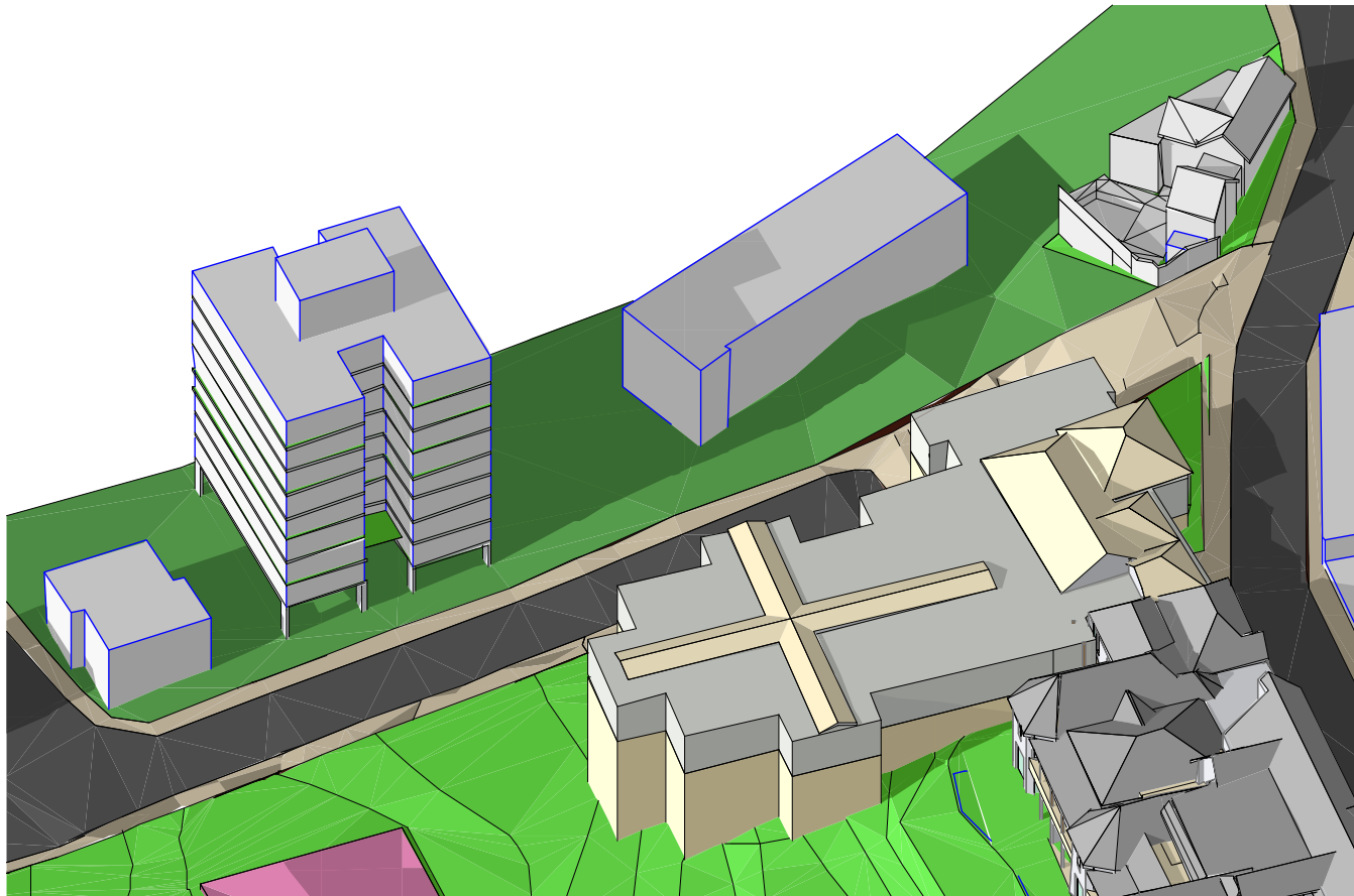
Existing Shadows - 21st June 10am
