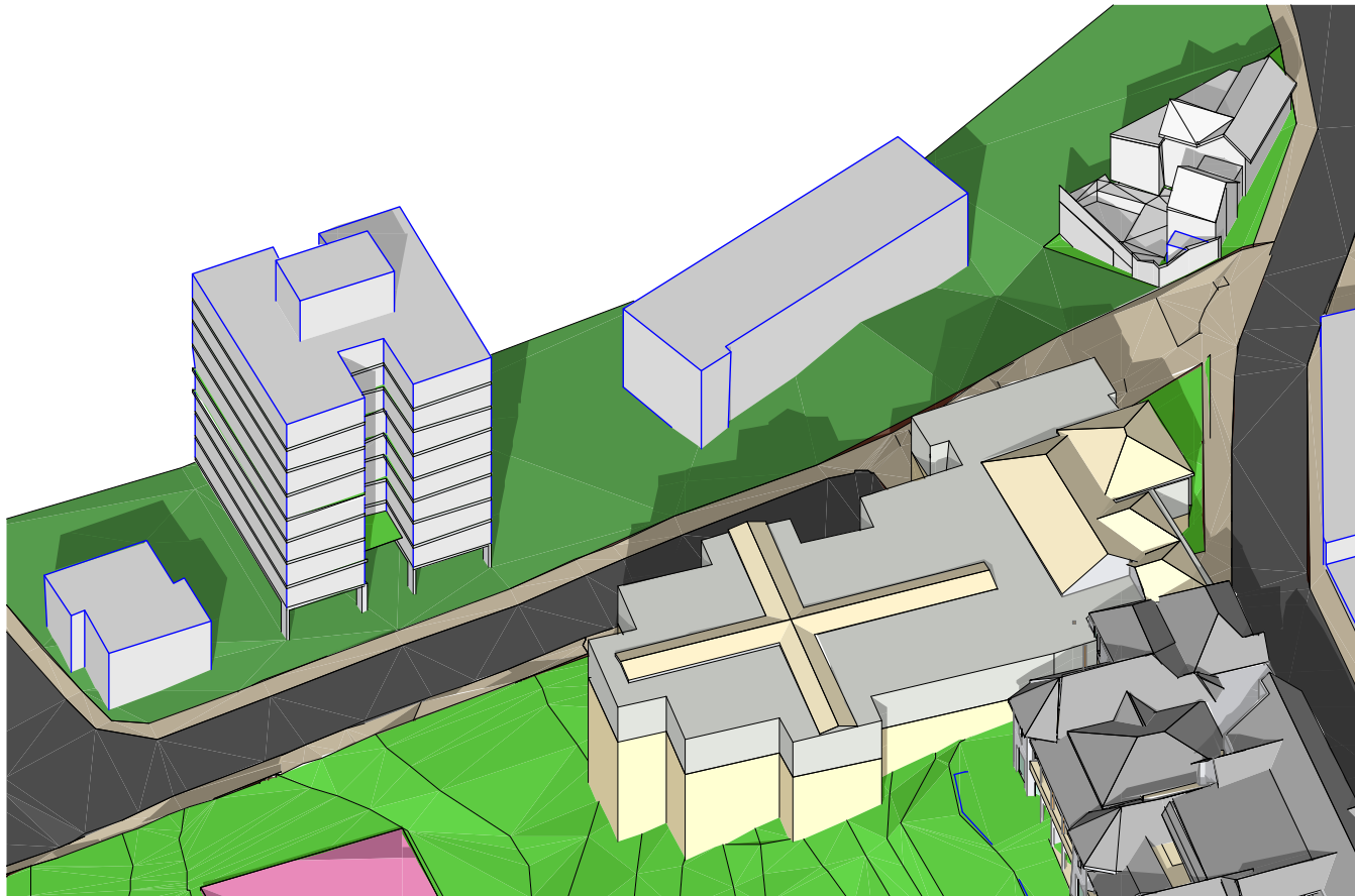
Existing Shadows - 21st June 1.30pm
