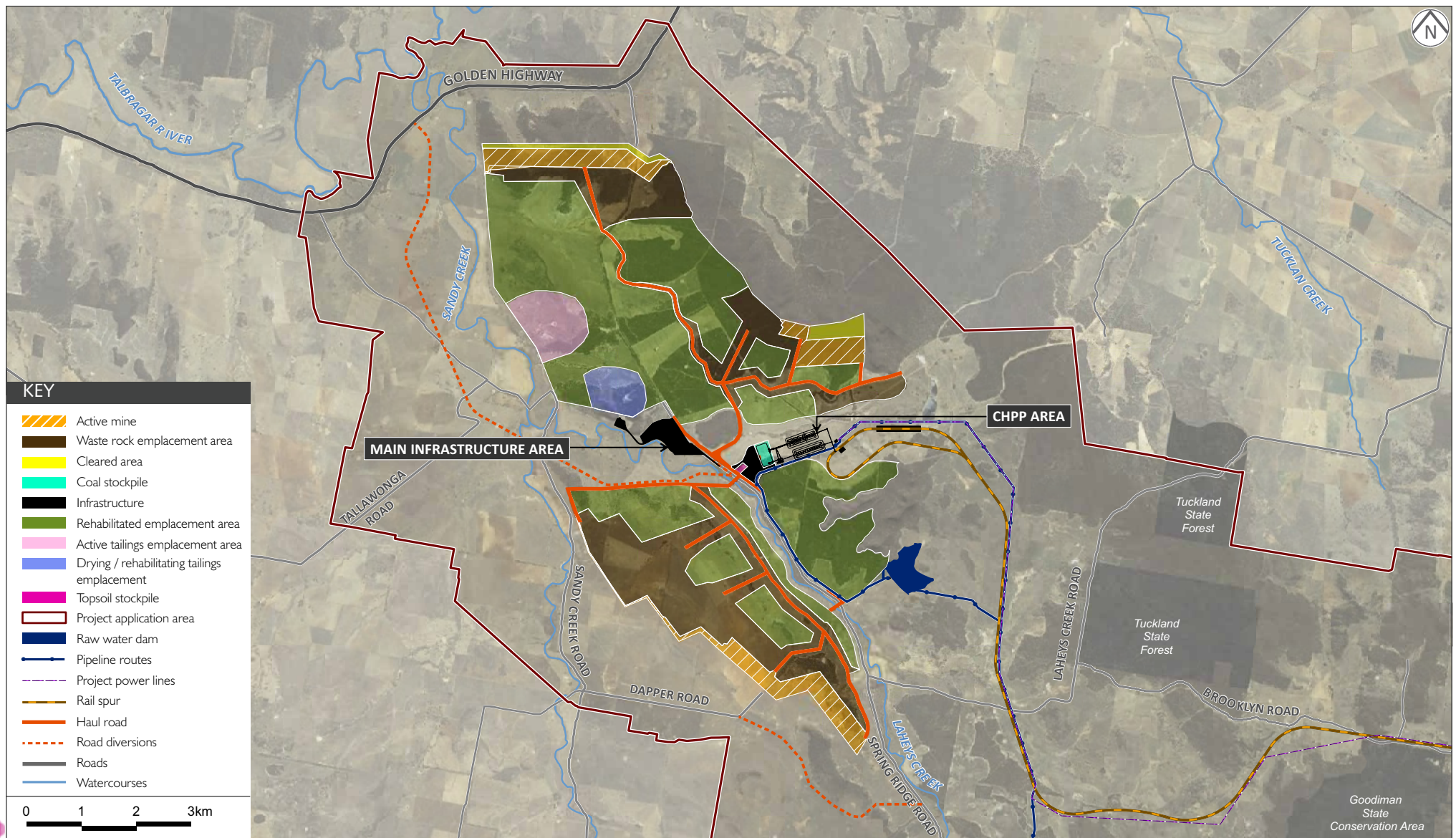
Indicative Mine Plan - Year 20
