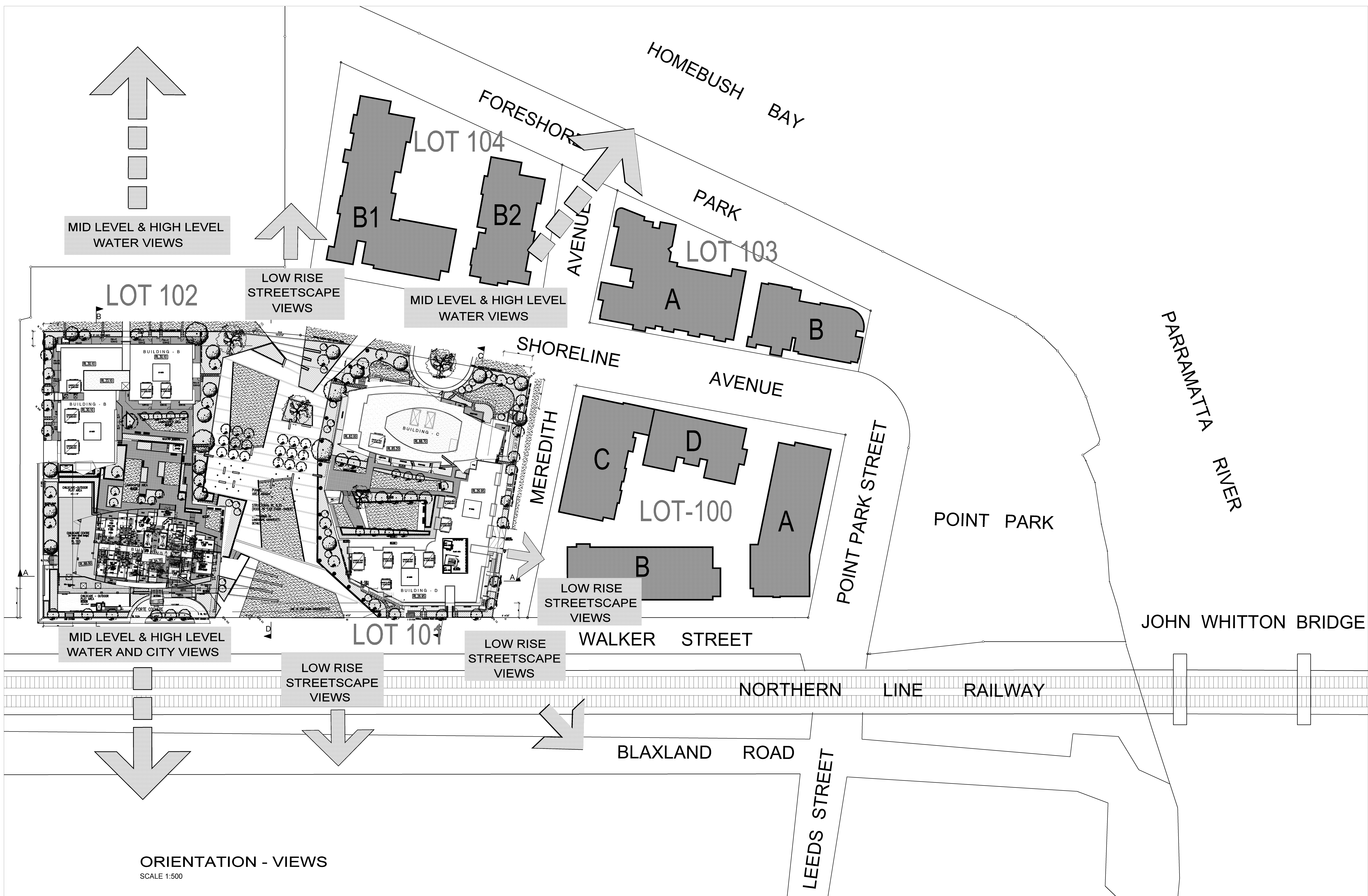
SITE ANALYSIS PLAN - 2 SCALE 1:200
