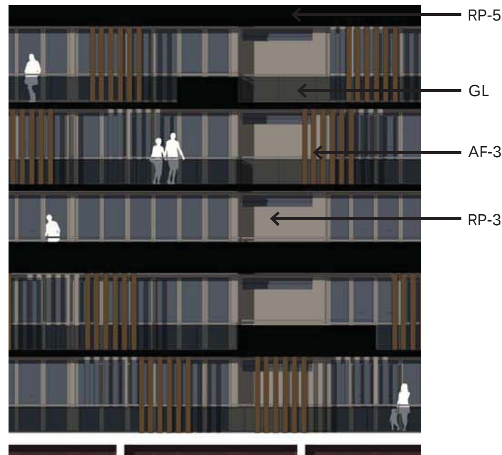
PARTIAL DETAIL ELEVATION
