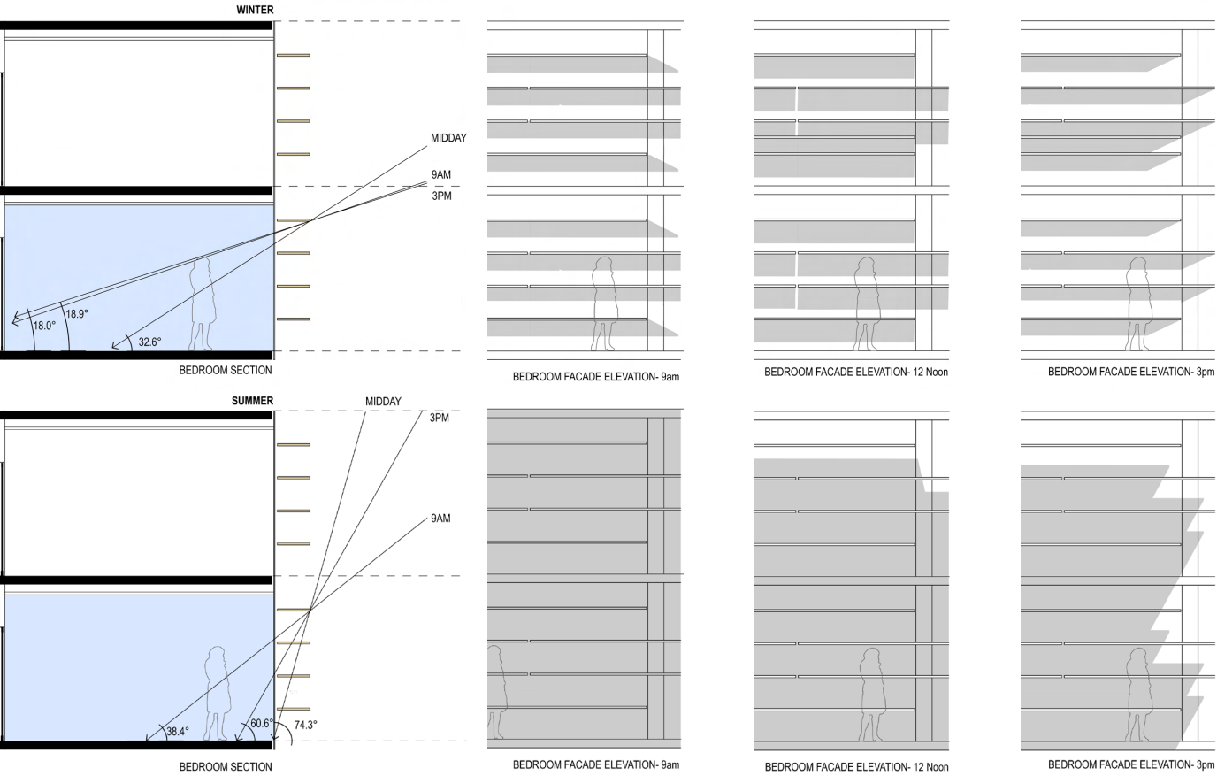
DIAGRAM: 17. CANTILEVERED FACADE SCREEN SHADING AND PRIVACY STUDIES
