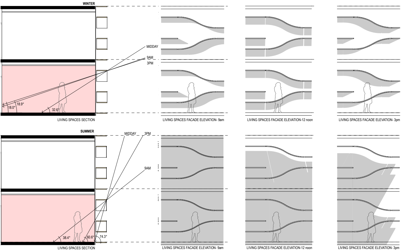
DIAGRAM: 16. CANTILEVERED FACADE SCREEN RENDER
