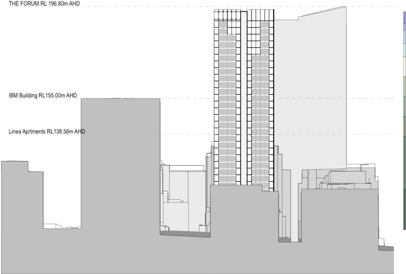
02 ELEVATION Mitchell St Elevation 1:1000
