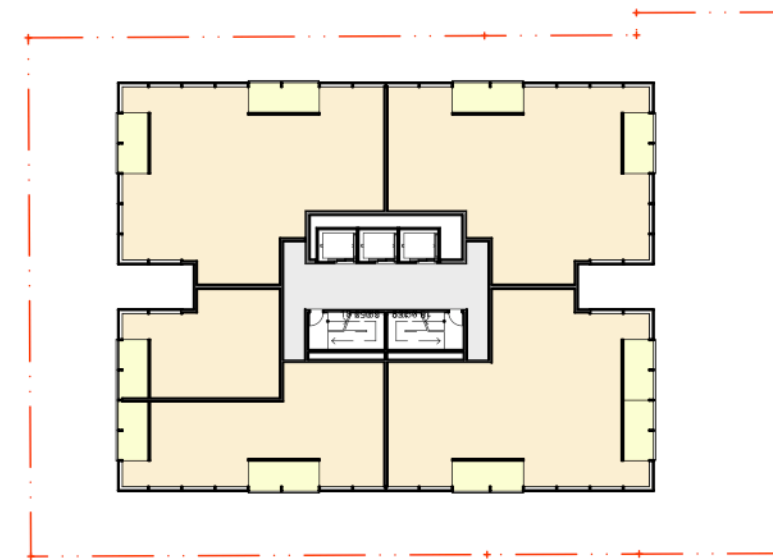
03 PLAN Typical High Tower L28-29 T2 1:500
