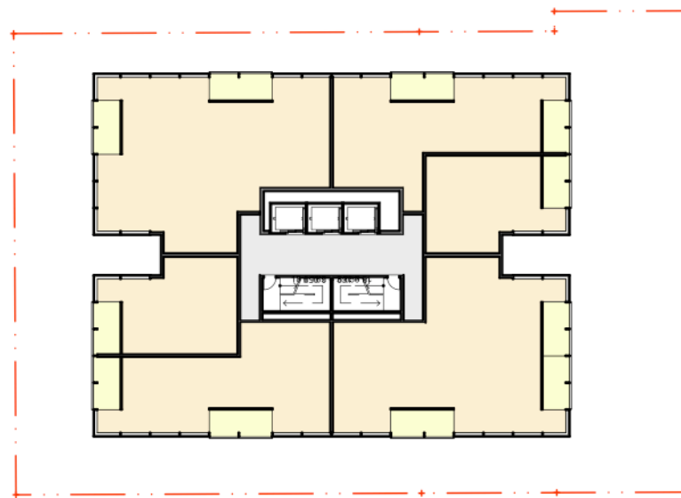
02 PLAN Typical High Tower L25-27 T1 1:500
