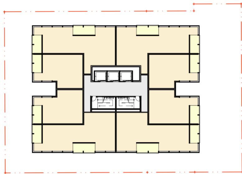
01 PLAN Typical Mid Tower L22-24 T3 1:500
