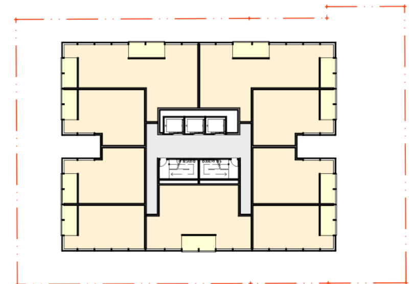
06 PLAN Typical Mid Tower L19-21 T2 1:500
