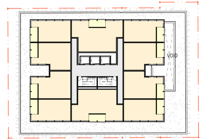
03 PLAN Typical Serviced Apartments L2-7 1:500
