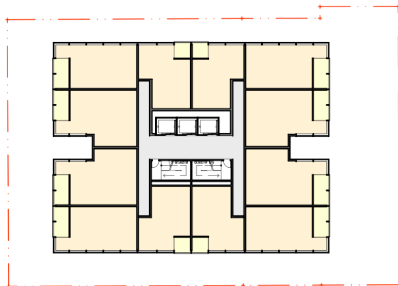
04 PLAN Typical Low Tower L8-15 1:500
