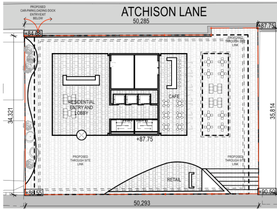
01 PLAN Ground Floor 1:500
