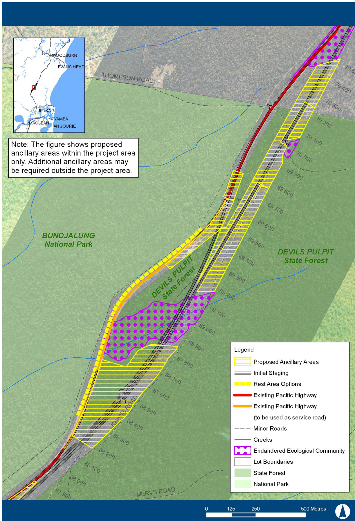
Figure 4-10b Possible locations for ancillary areas (initial staging) (Ch 68000-70500)
