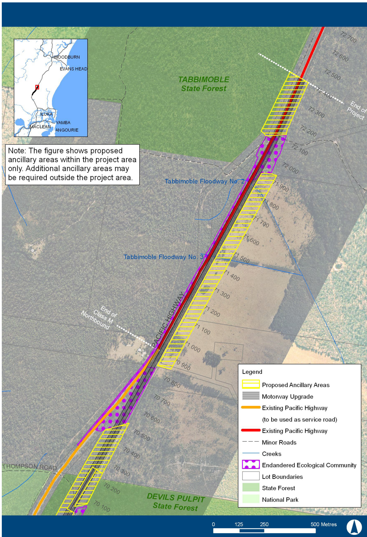
Figure 4-9c Possible locations for ancillary areas (motorway upgrade) (Ch 70500-72500)
