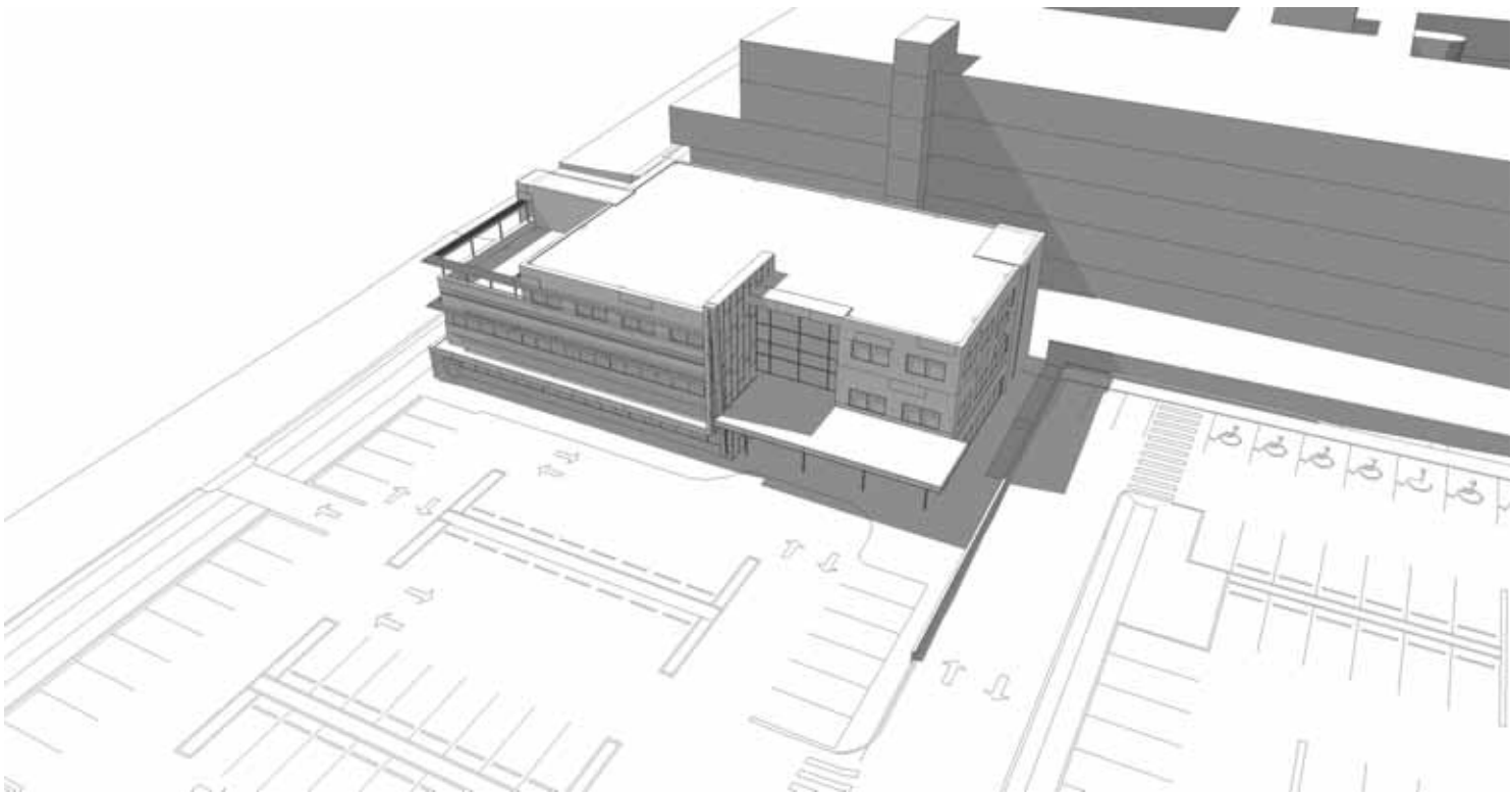
NORTH WEST PERSPECTIVE OF SUNSHADING AT 9AM 21ST OF DECEMBER
