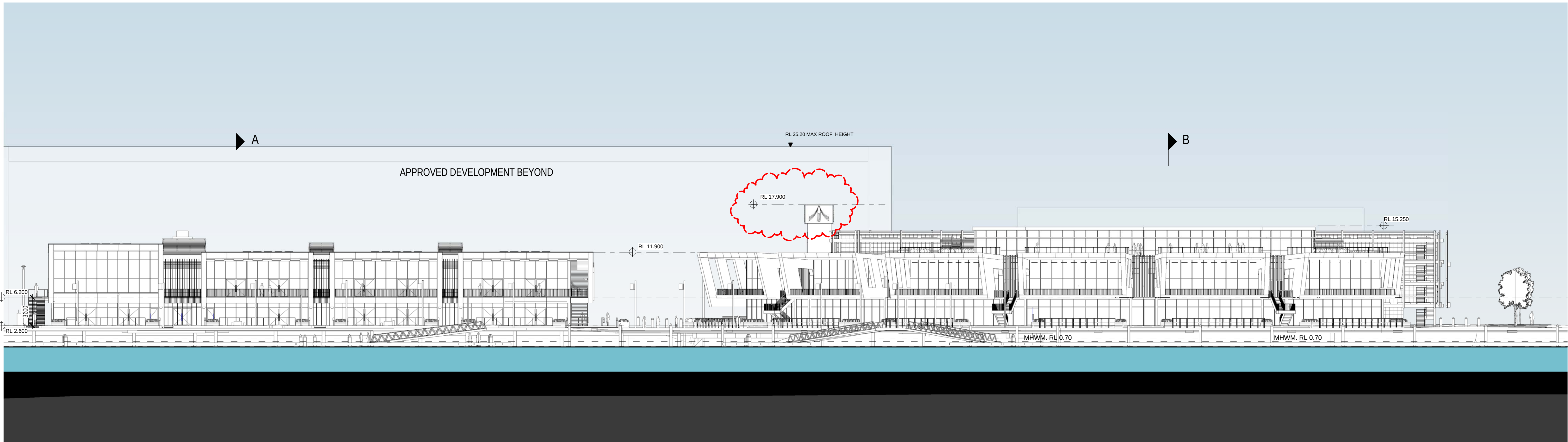
1 SOUTH ELEVATION 1 : 250
