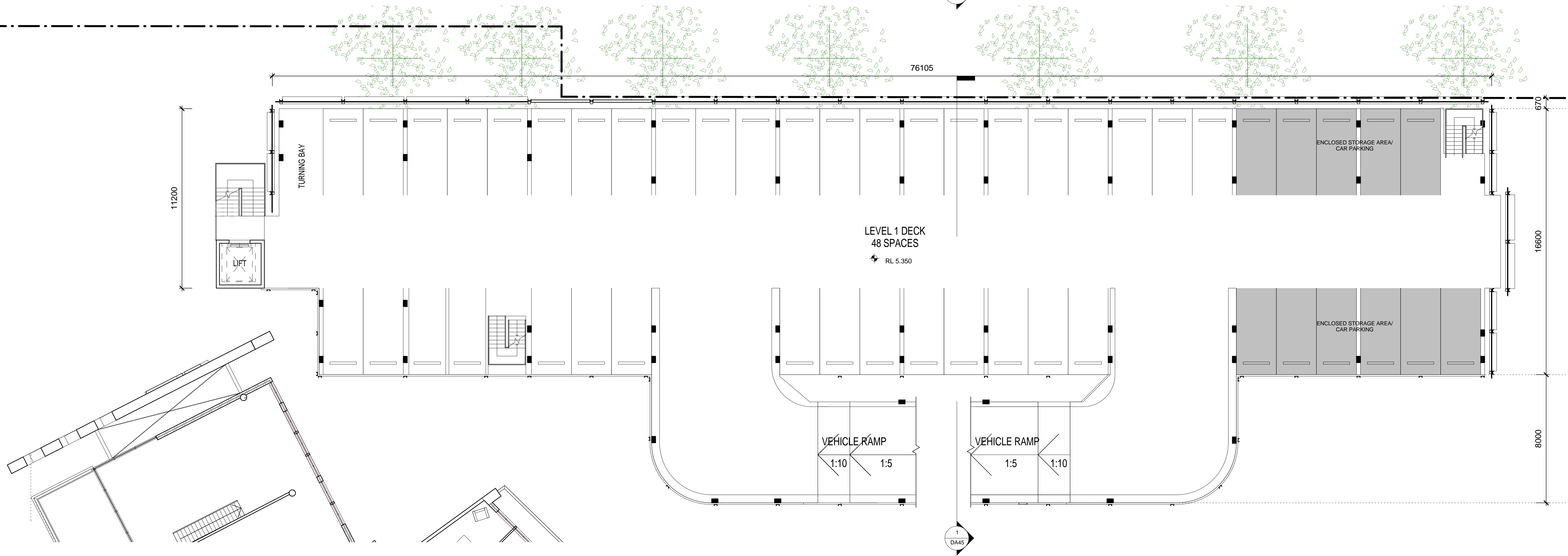
1 First Floor Plan - Carpark 1 : 125
