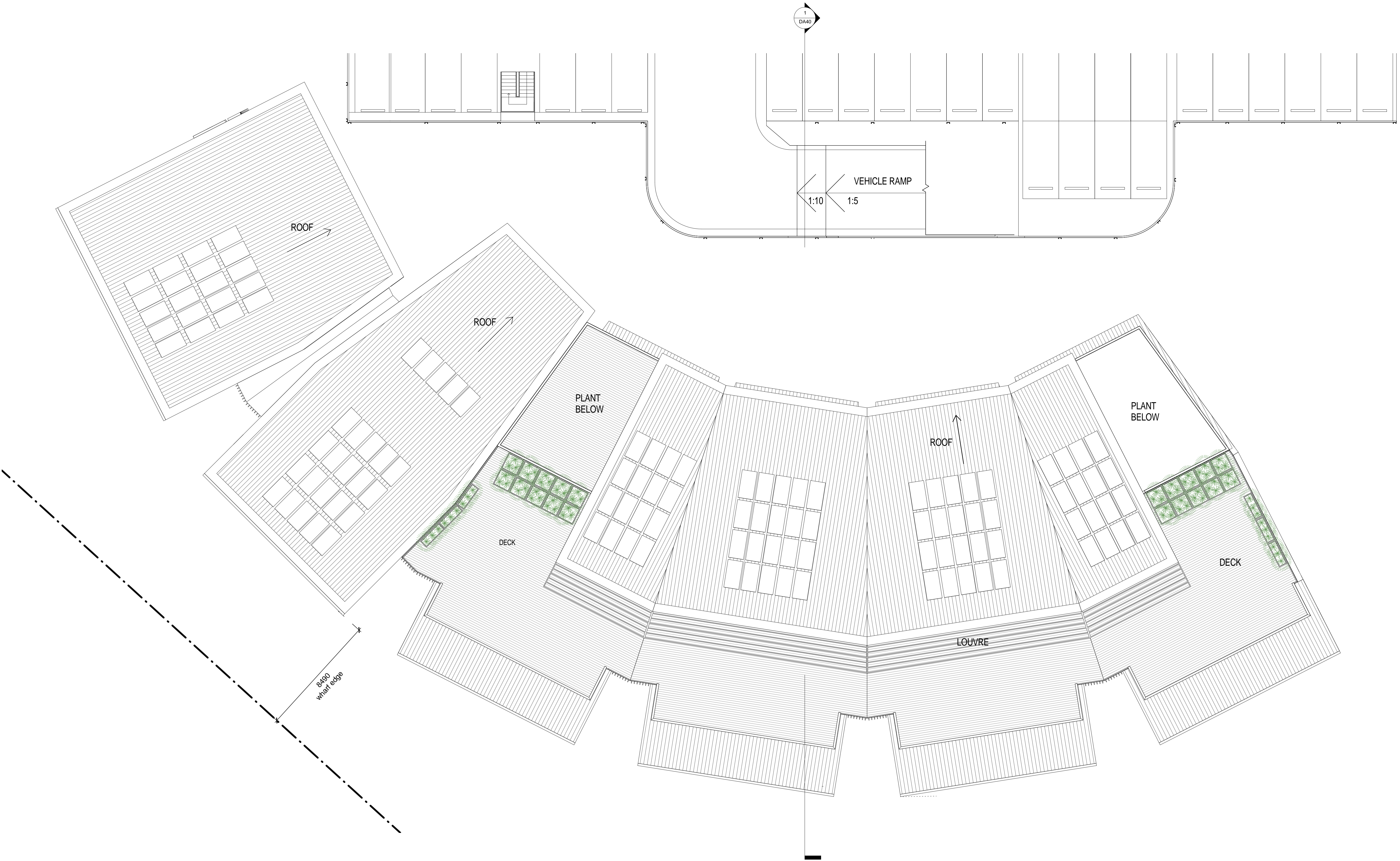
1 Roof Plan - East Building 1 : 125
