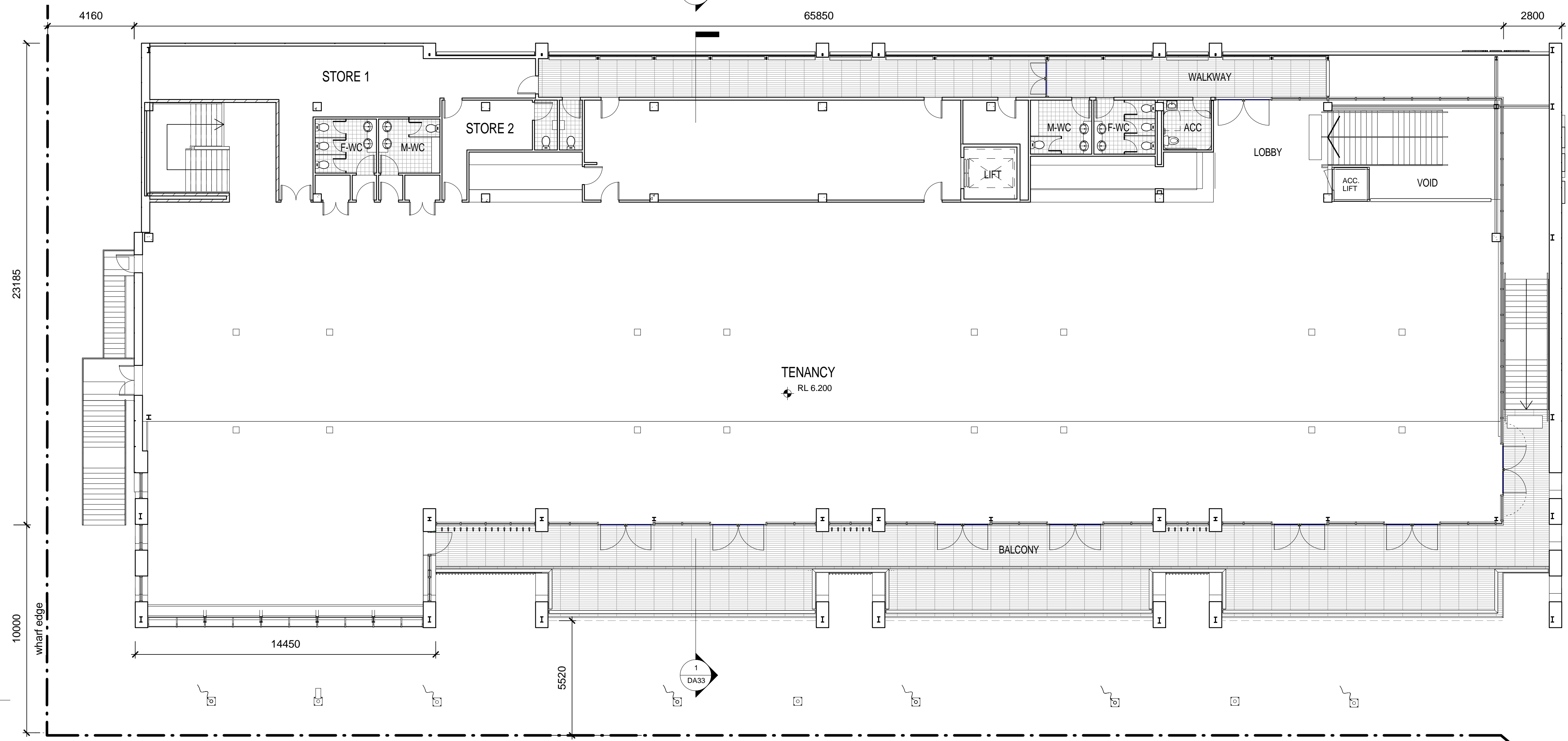
1 First Floor Plan - West Building 1 : 125
