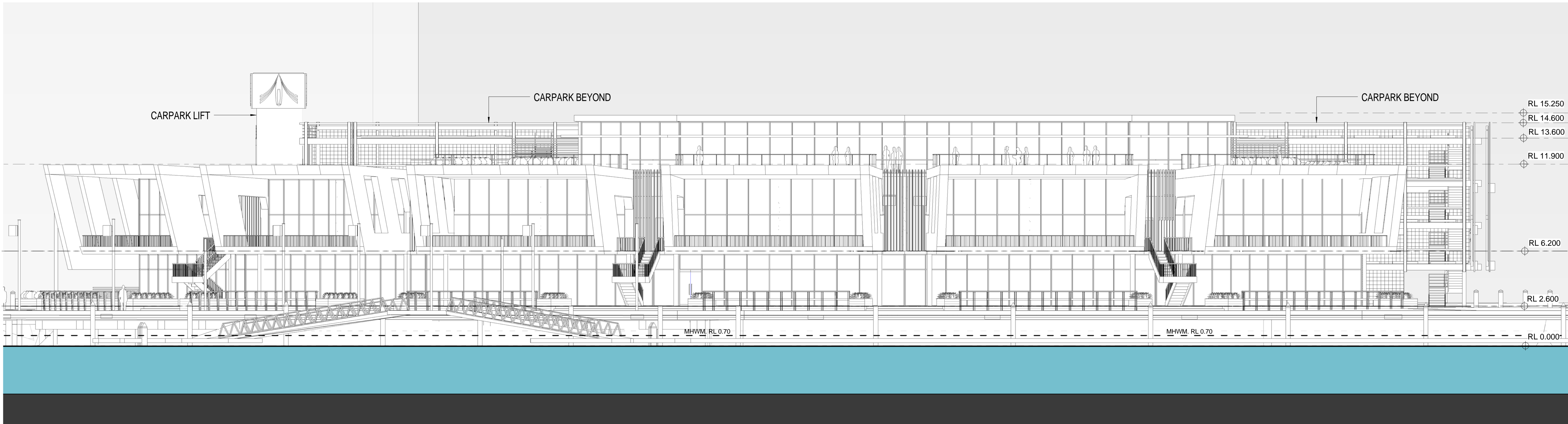
2 South Elevation - East Building 1 : 125
