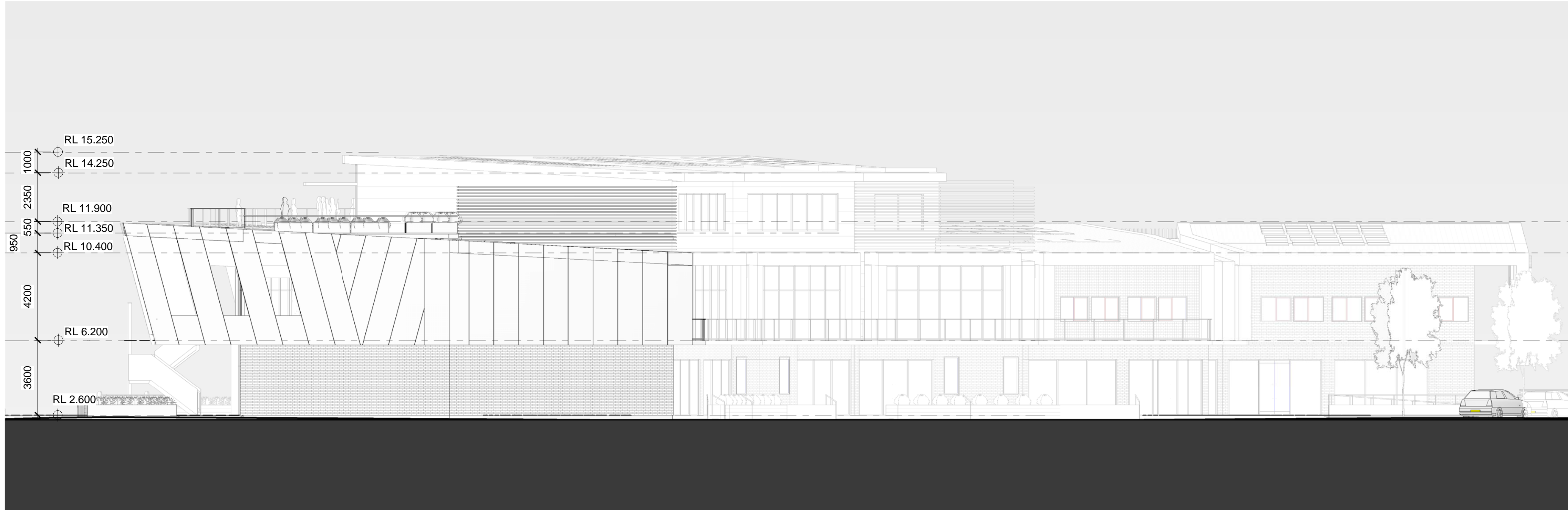
1 East Elevation - East Building 1 : 125
