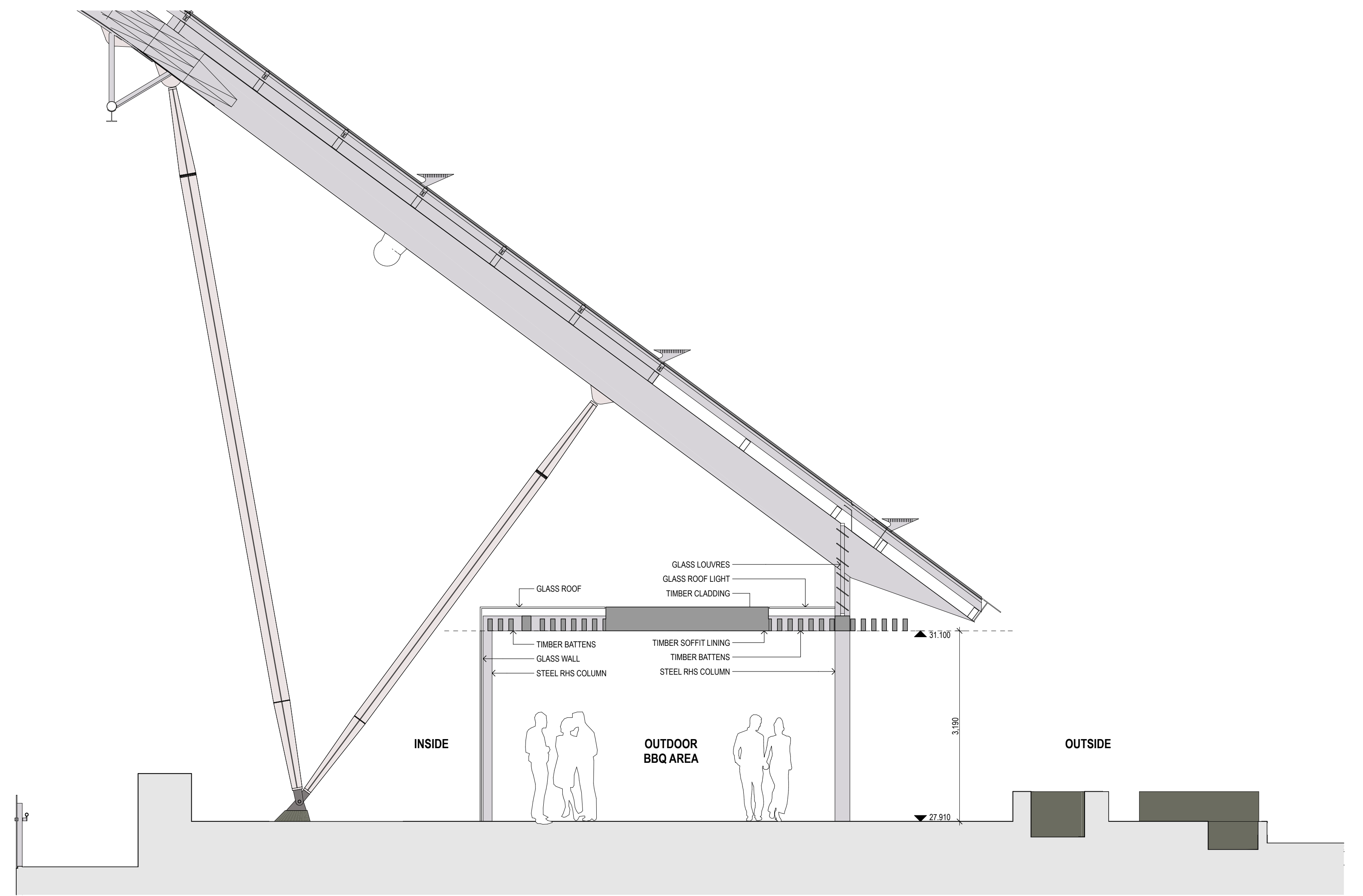
2 Level 6 Terrace - Section 3 1:50
