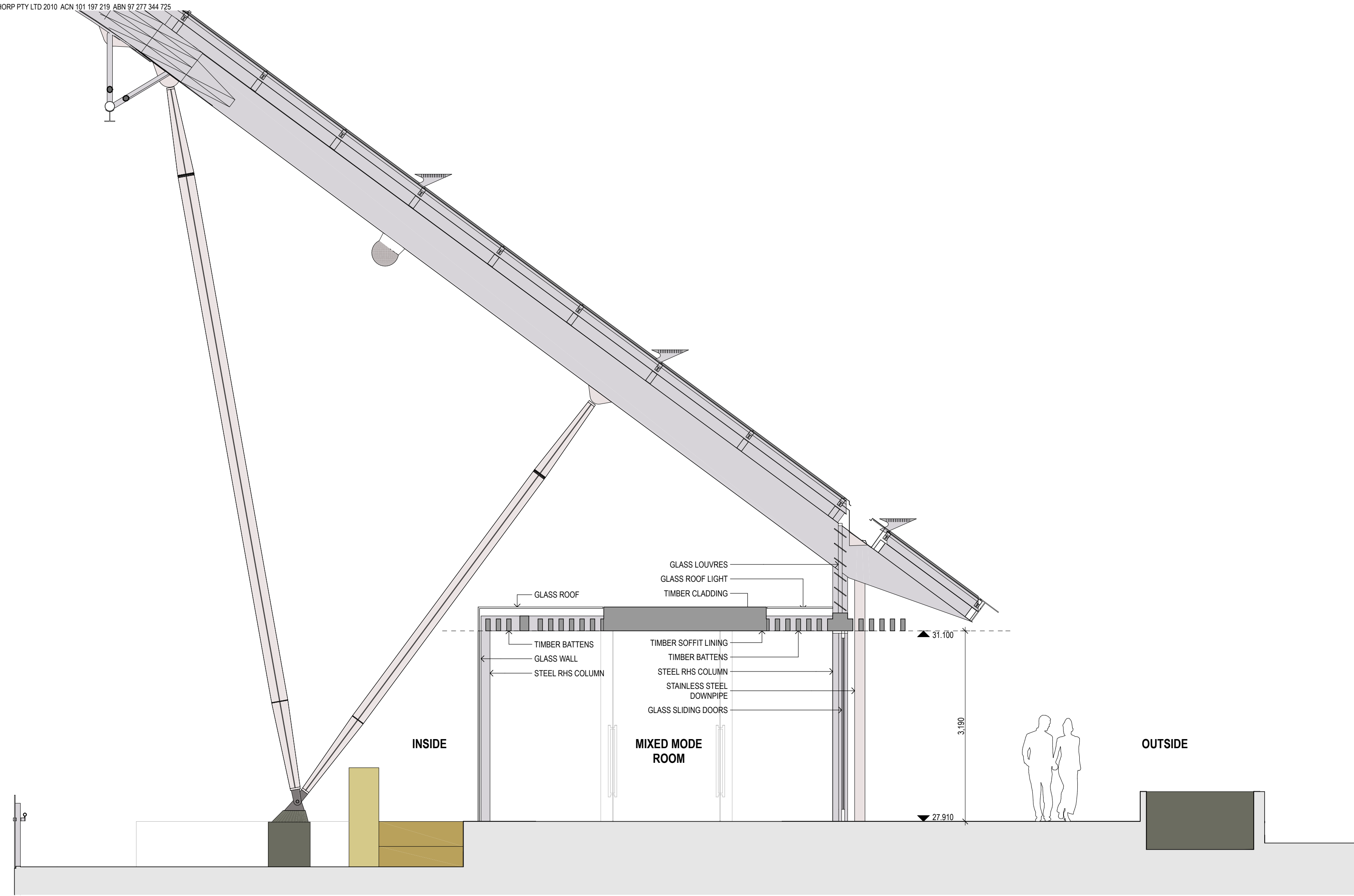
1 Level 6 Terrace - Section 2 1:50
