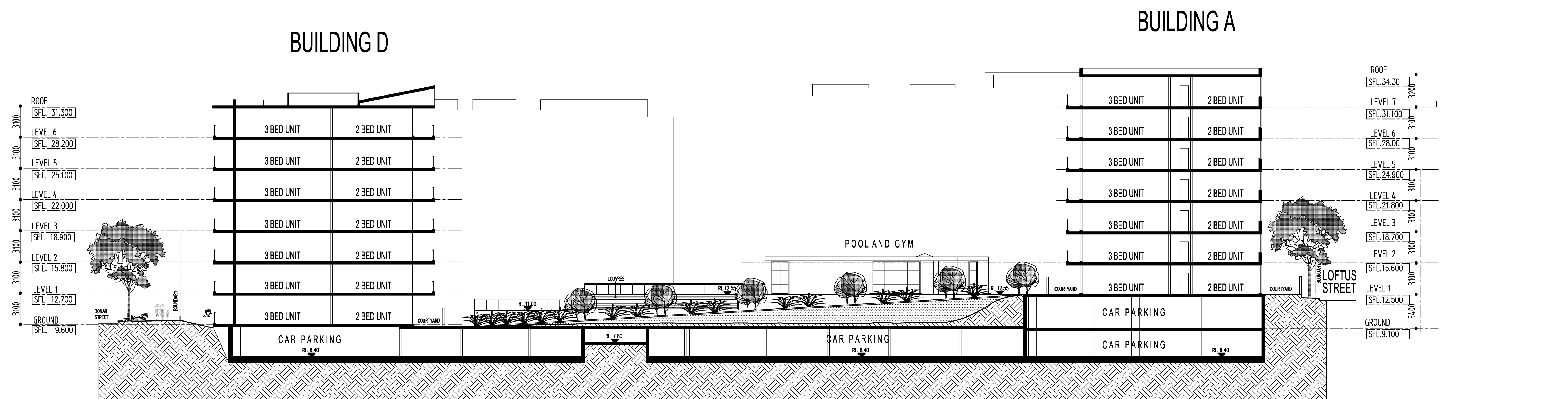
SECTION C-C
