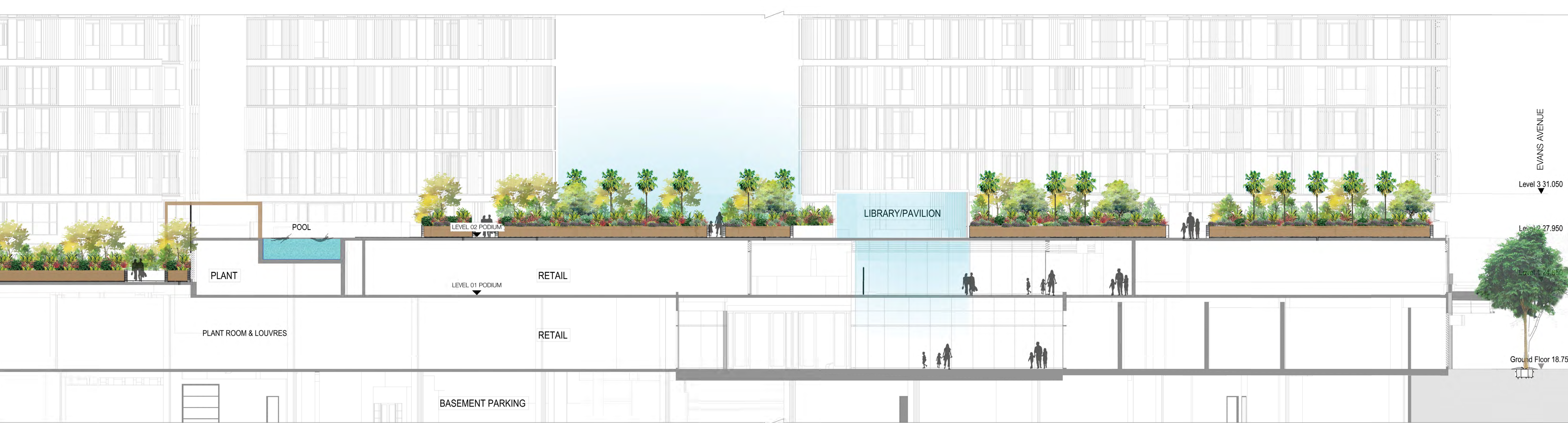
SECTION AA (2/2) SCALE 1:100
