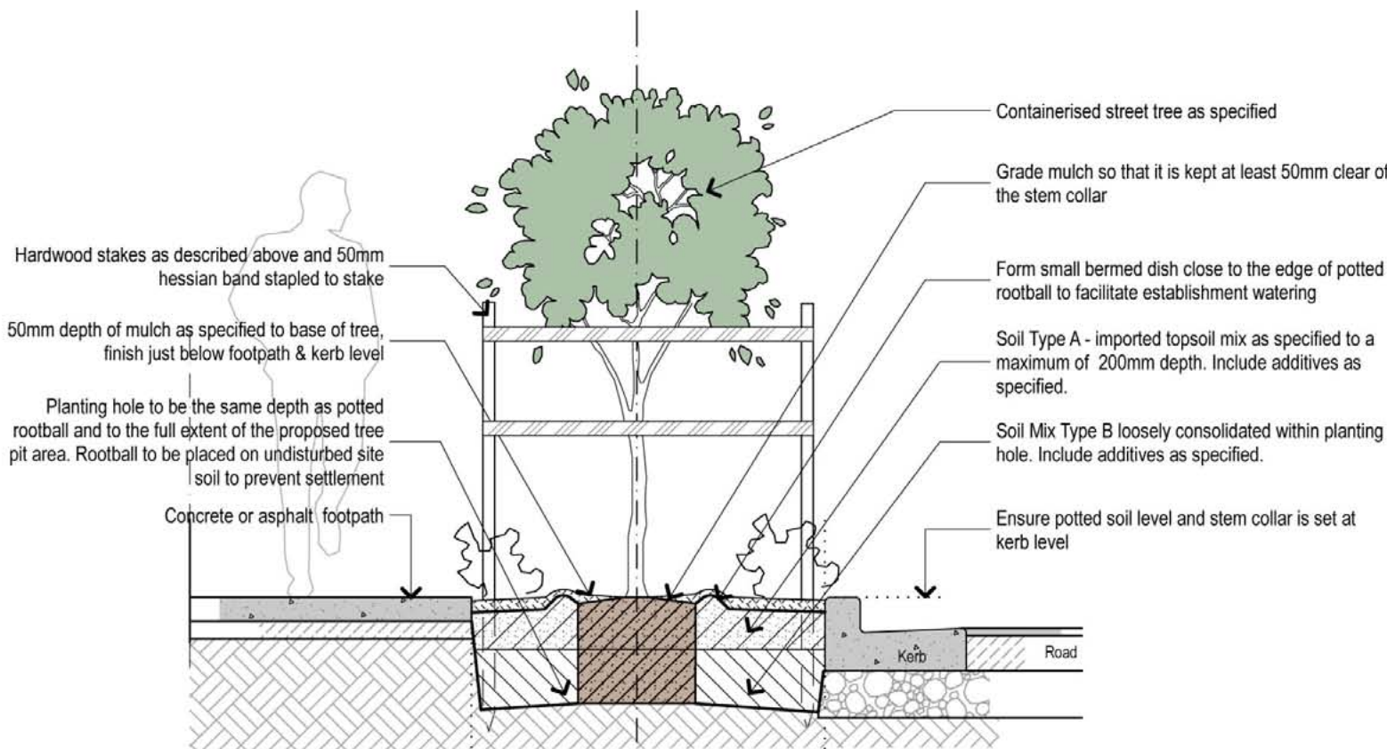
SECTION
