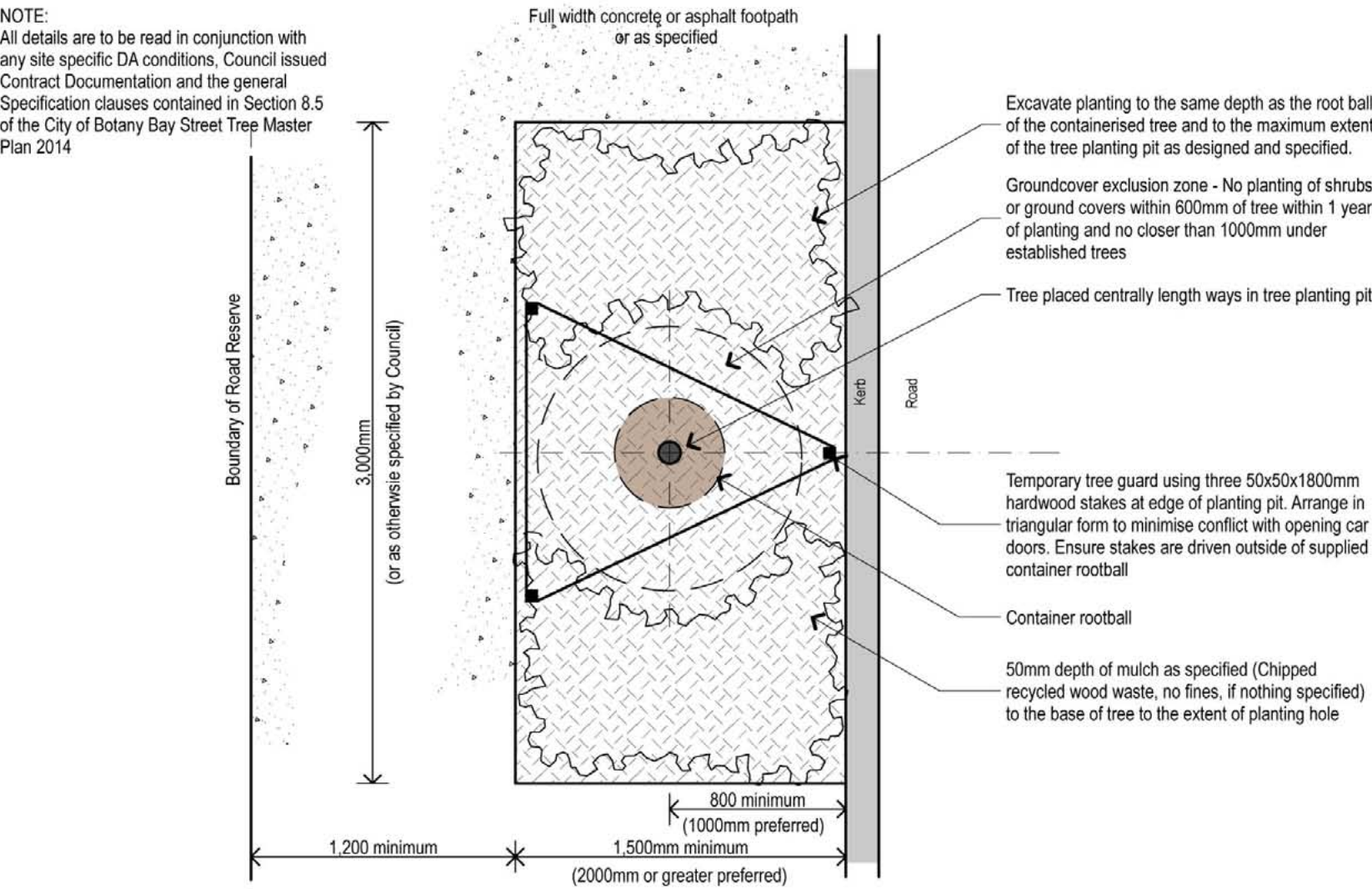
PLAN
