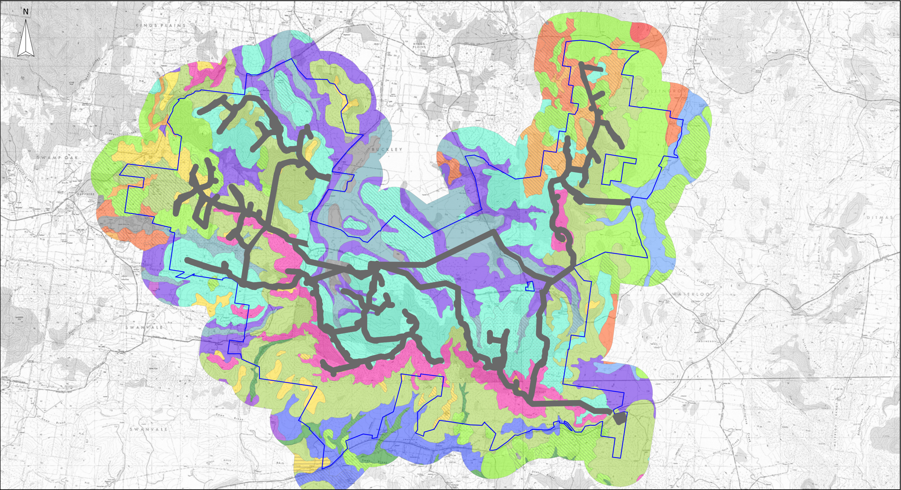
FIGURE 6: SOIL LANDSCAPES
