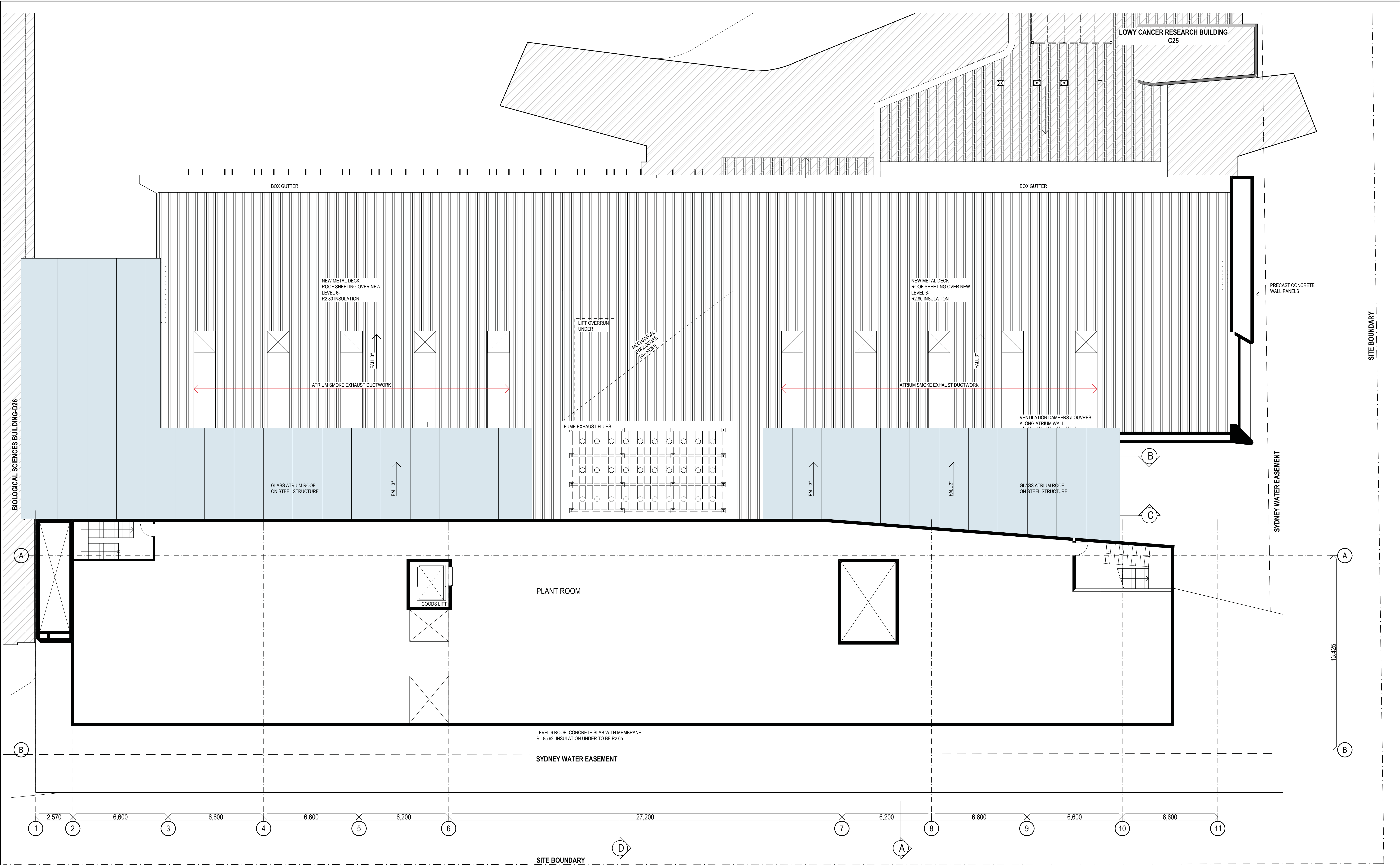
1 Level 7 1:100
