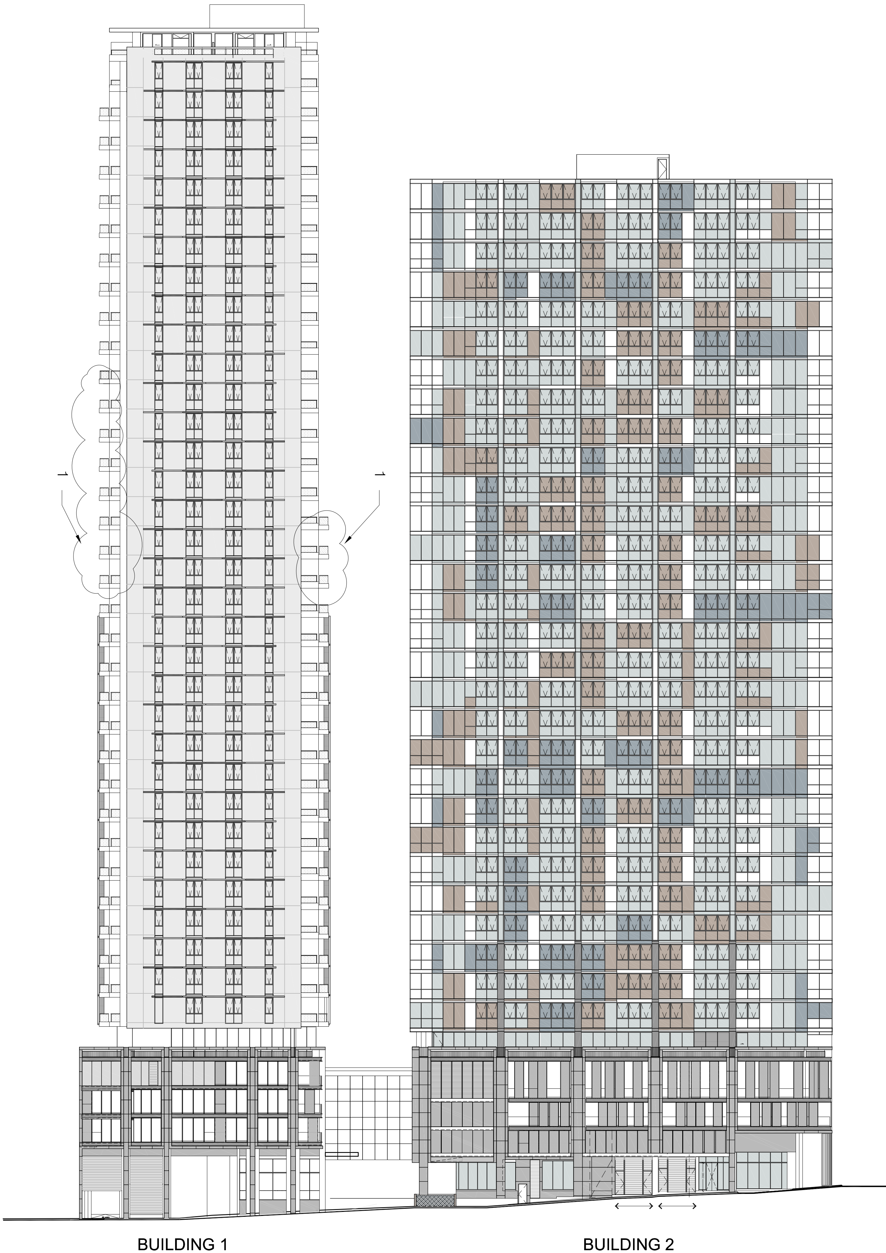
1 ELEVATION-NORTH 1:250
