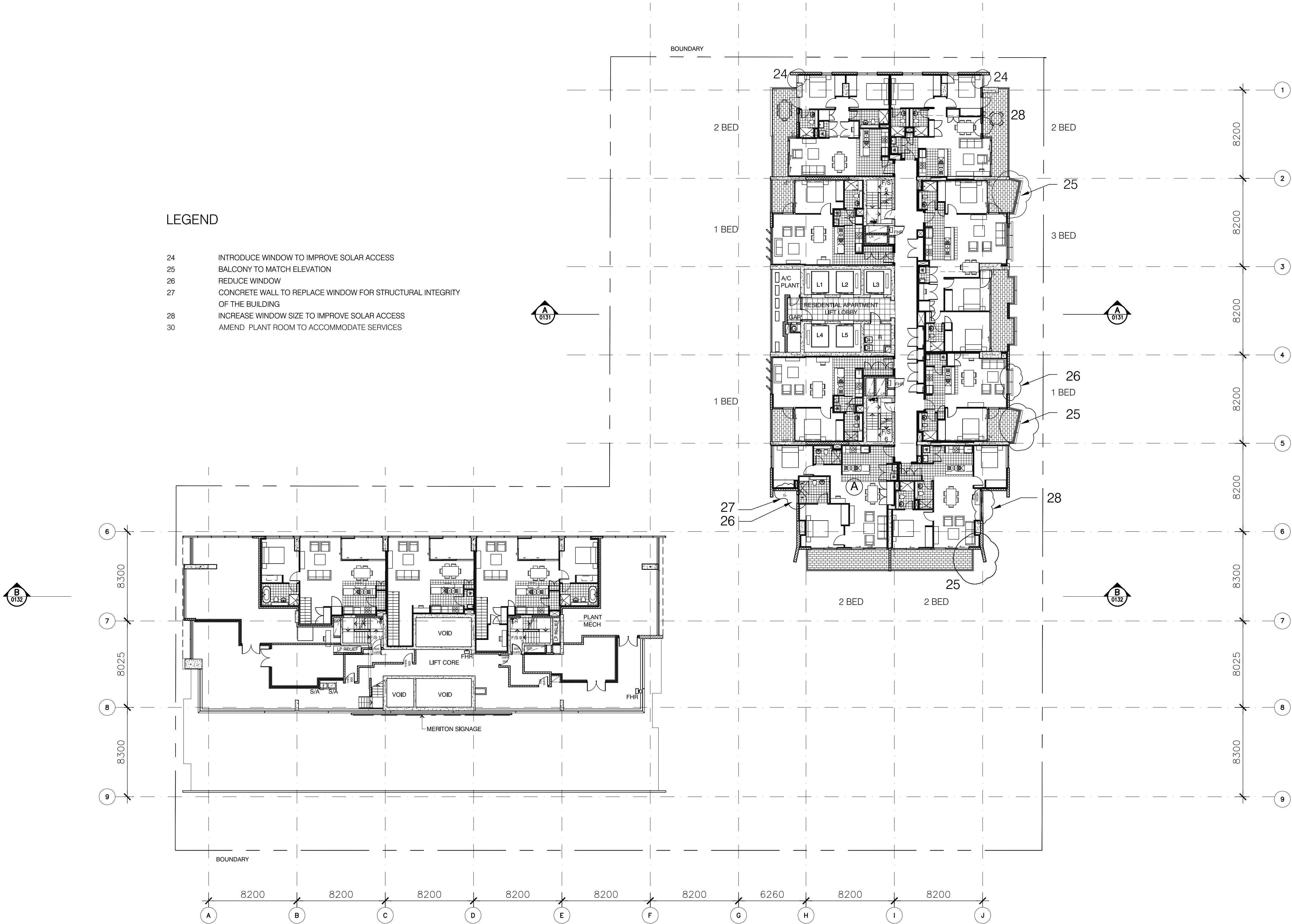
01 SERVICED APARTMENT – LEVEL 33 1:200
