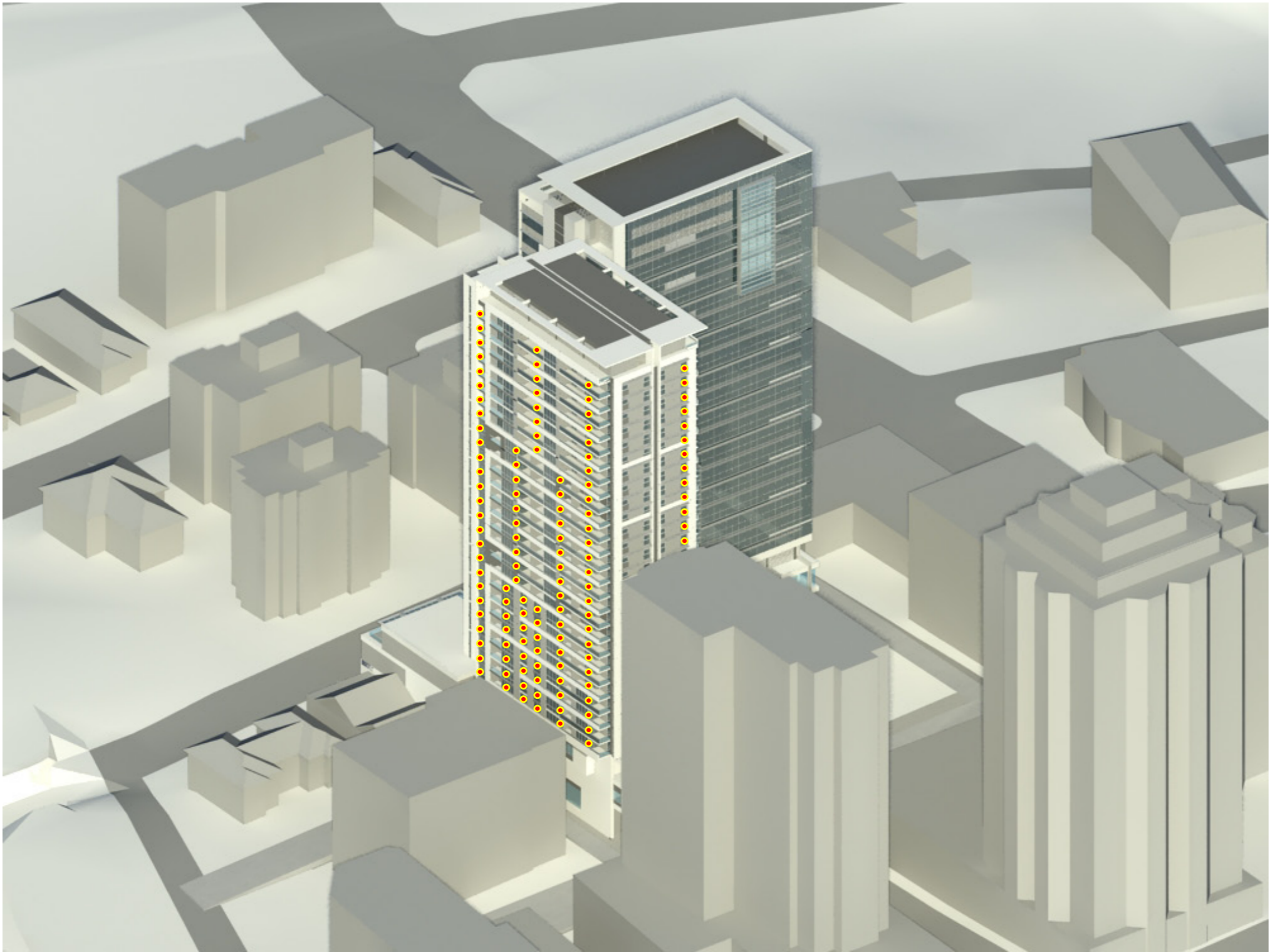
June 21, 11 am (Proposed Solar Access Diagram)
