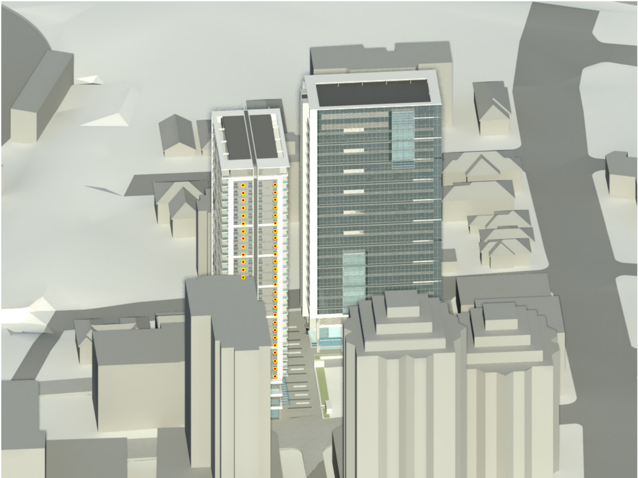
June 21, 1 pm (Proposed Solar Access Diagram)
