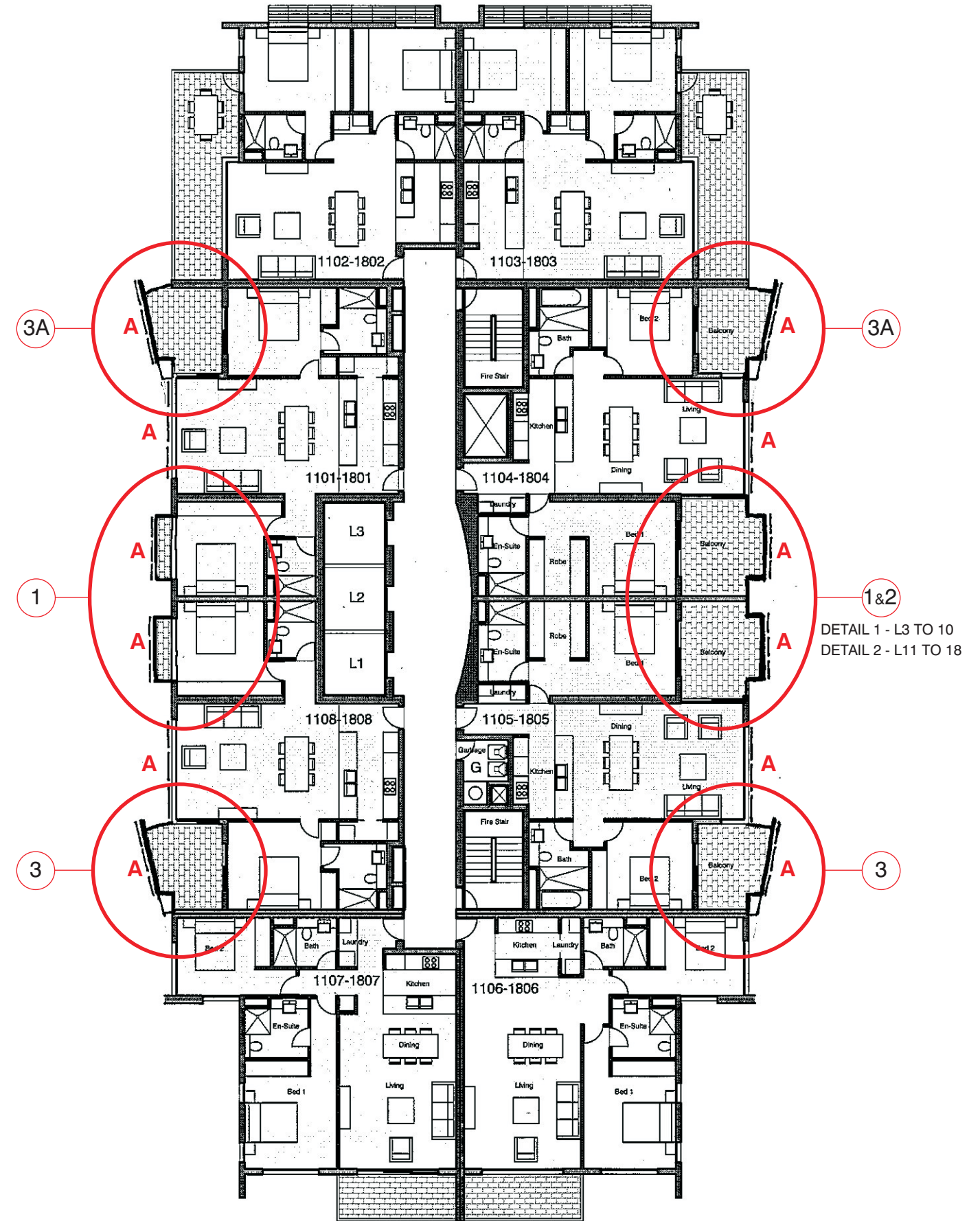
TYPICAL FLOOR PLAN (LEVELS 11-18 SHOWN)
