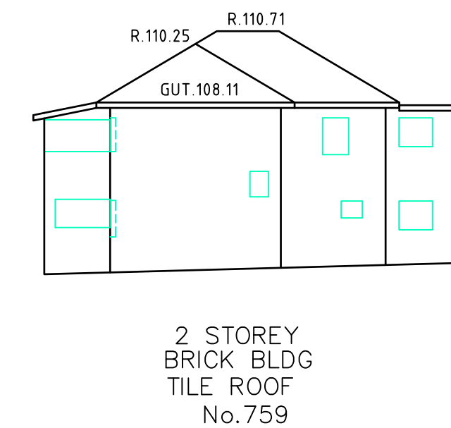
ELEVATION 2-2
