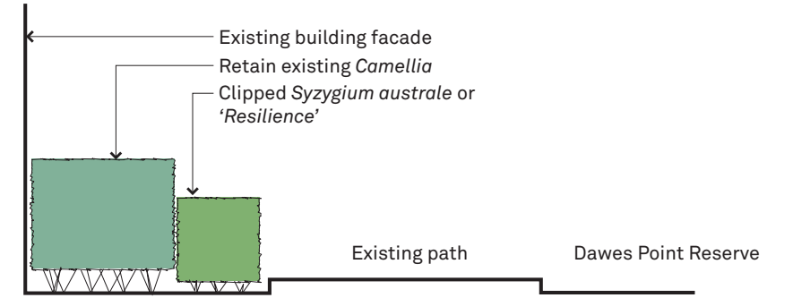
SECTION B: GROUND LEVEL PLANTING BED DAWES POINT RESERVE
