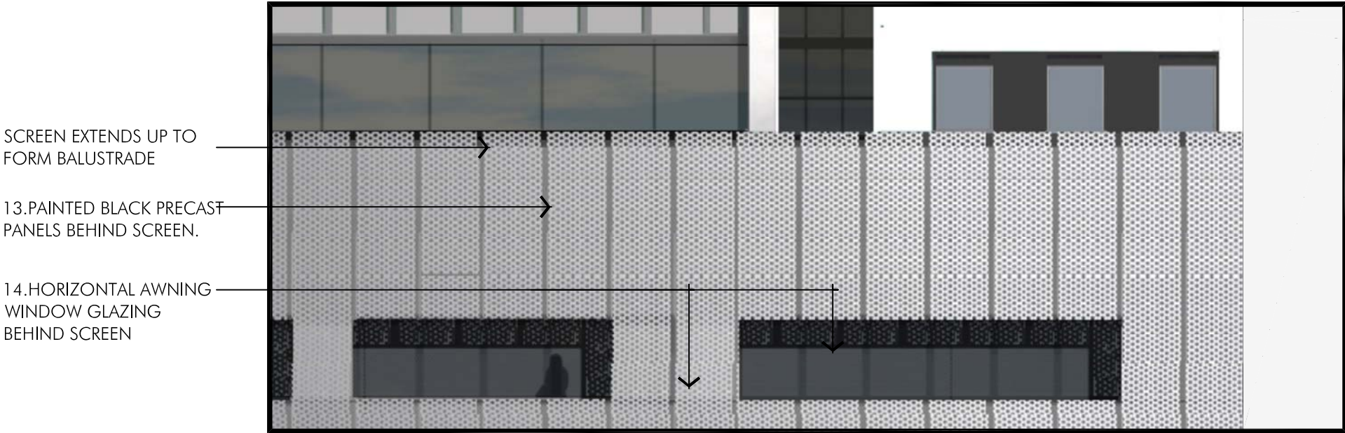
UPN: EAST PART ELEVATION
