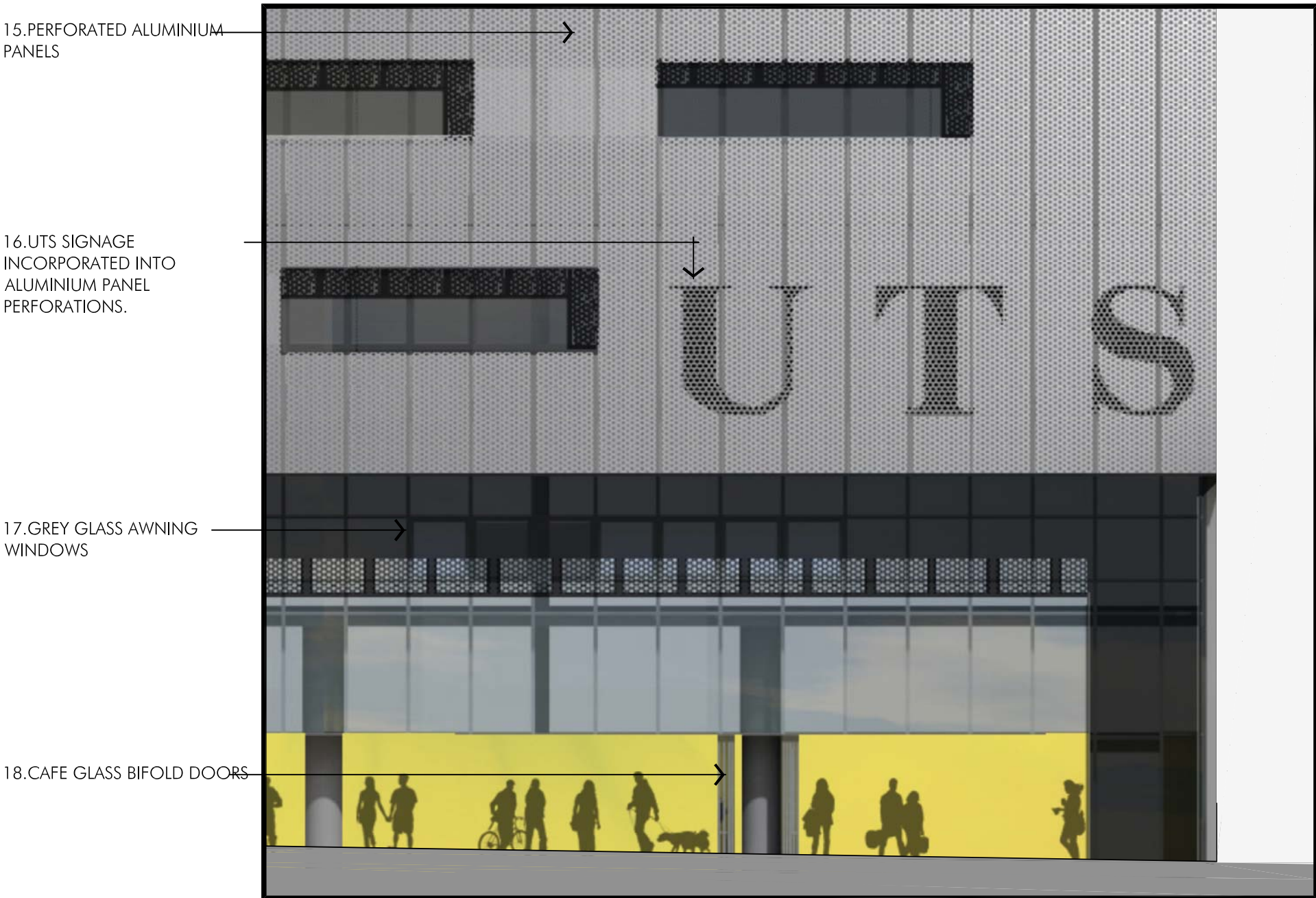
UPN: EAST LOWER PART ELEVATION
