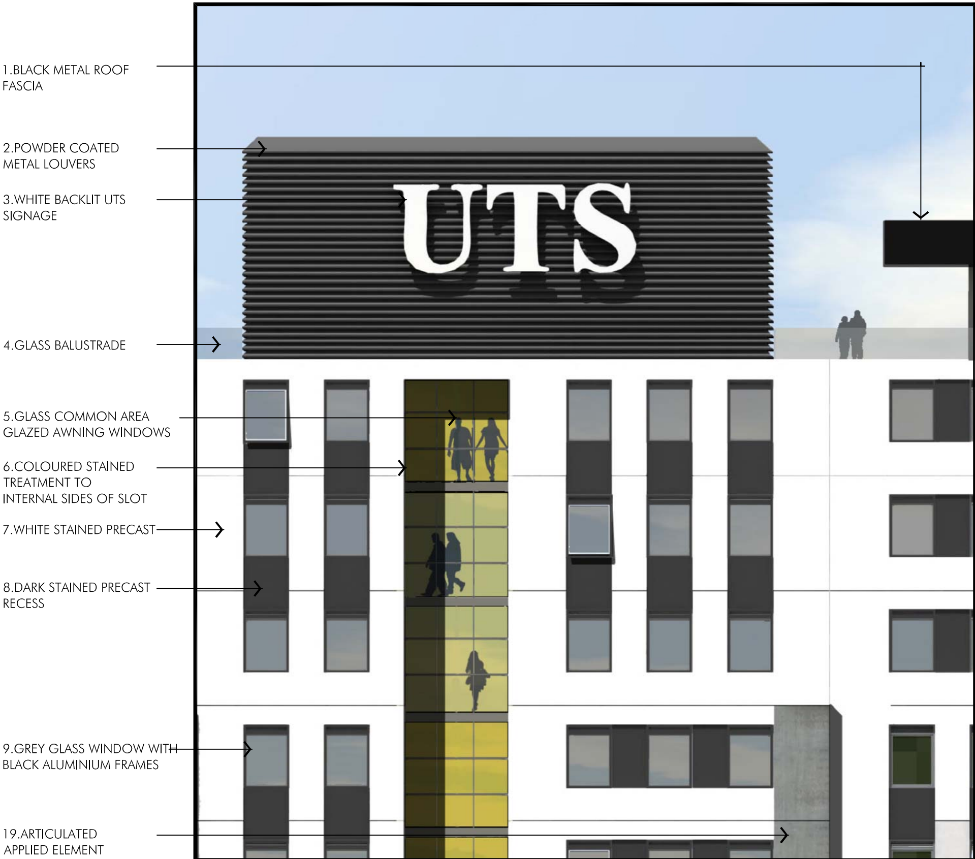
HARRIS STREET: WEST PART ELEVATION
