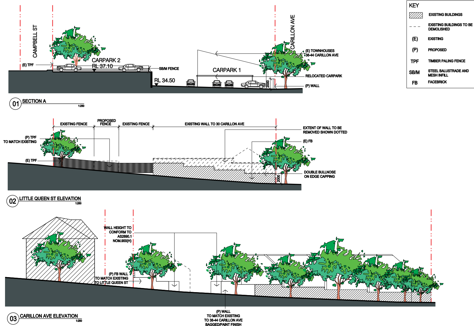
Figure PA 3120: Site B Elevations and Sections
