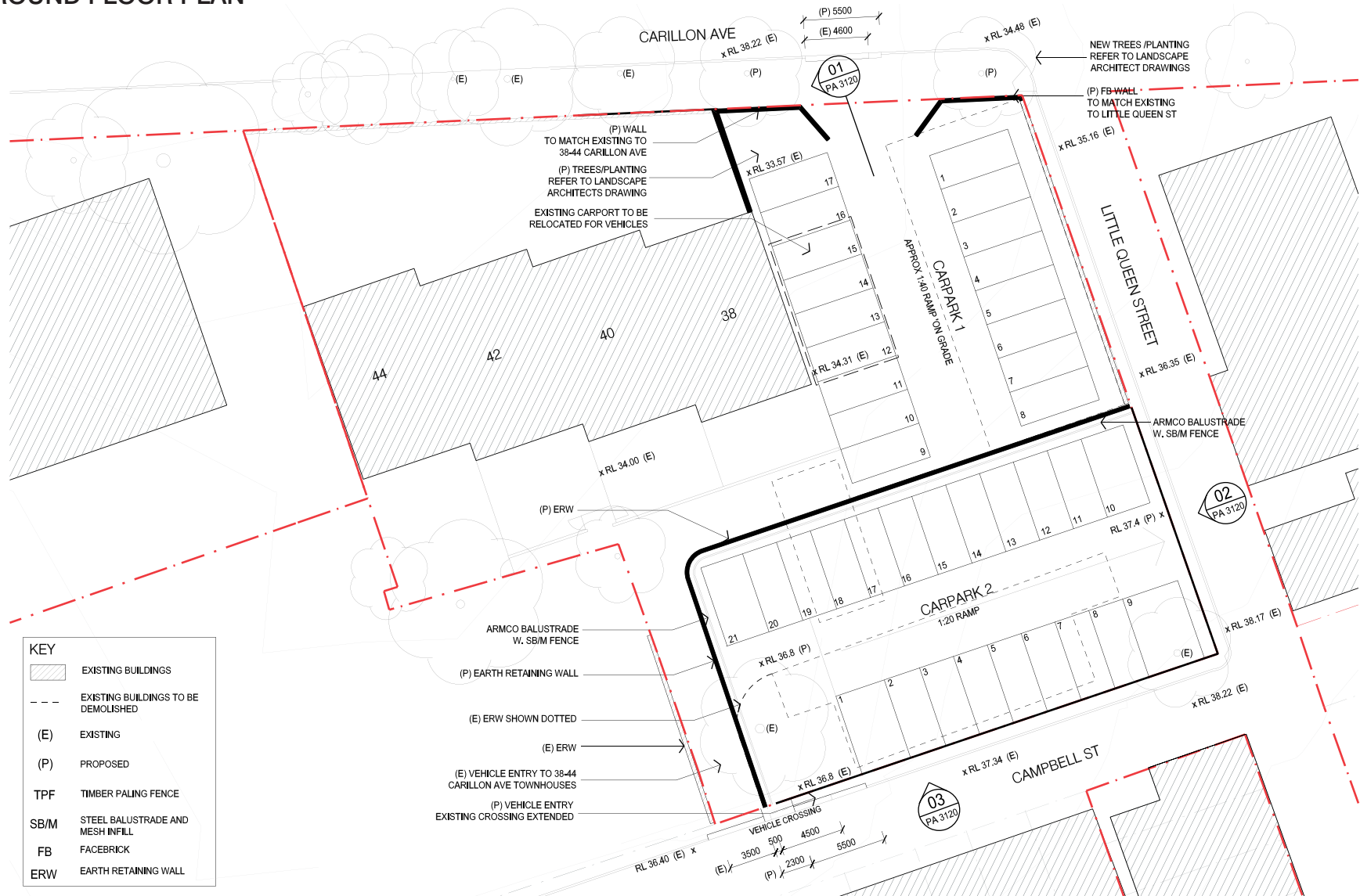
Figure PA 2120: Site B Ground Floor Plan
