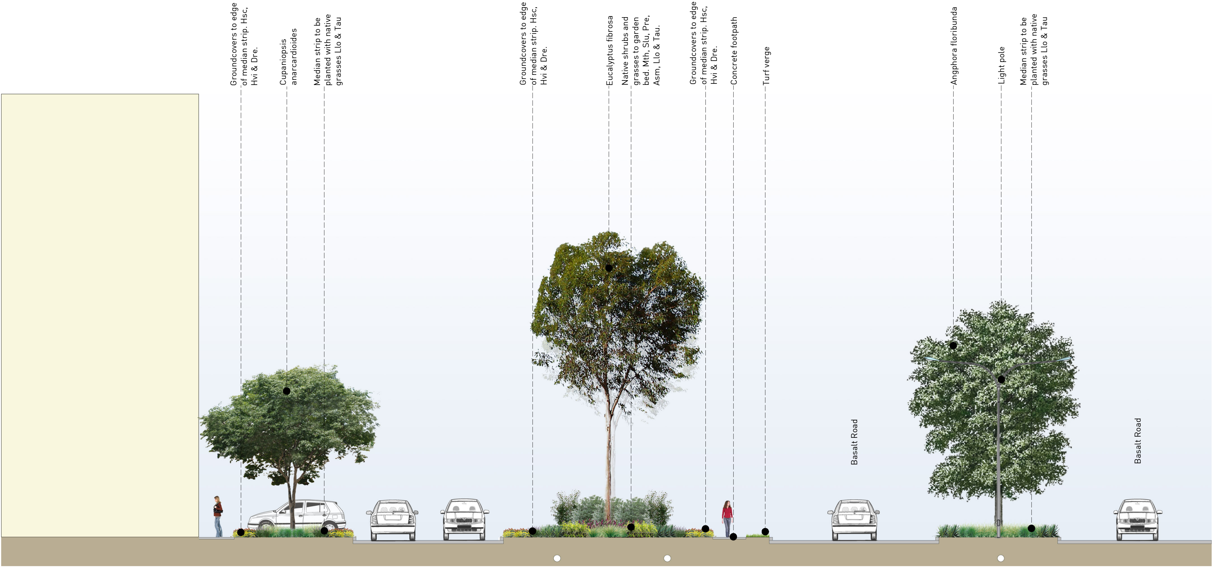
01 Section 1 : Basalt Road L01 1:100 @ A1
