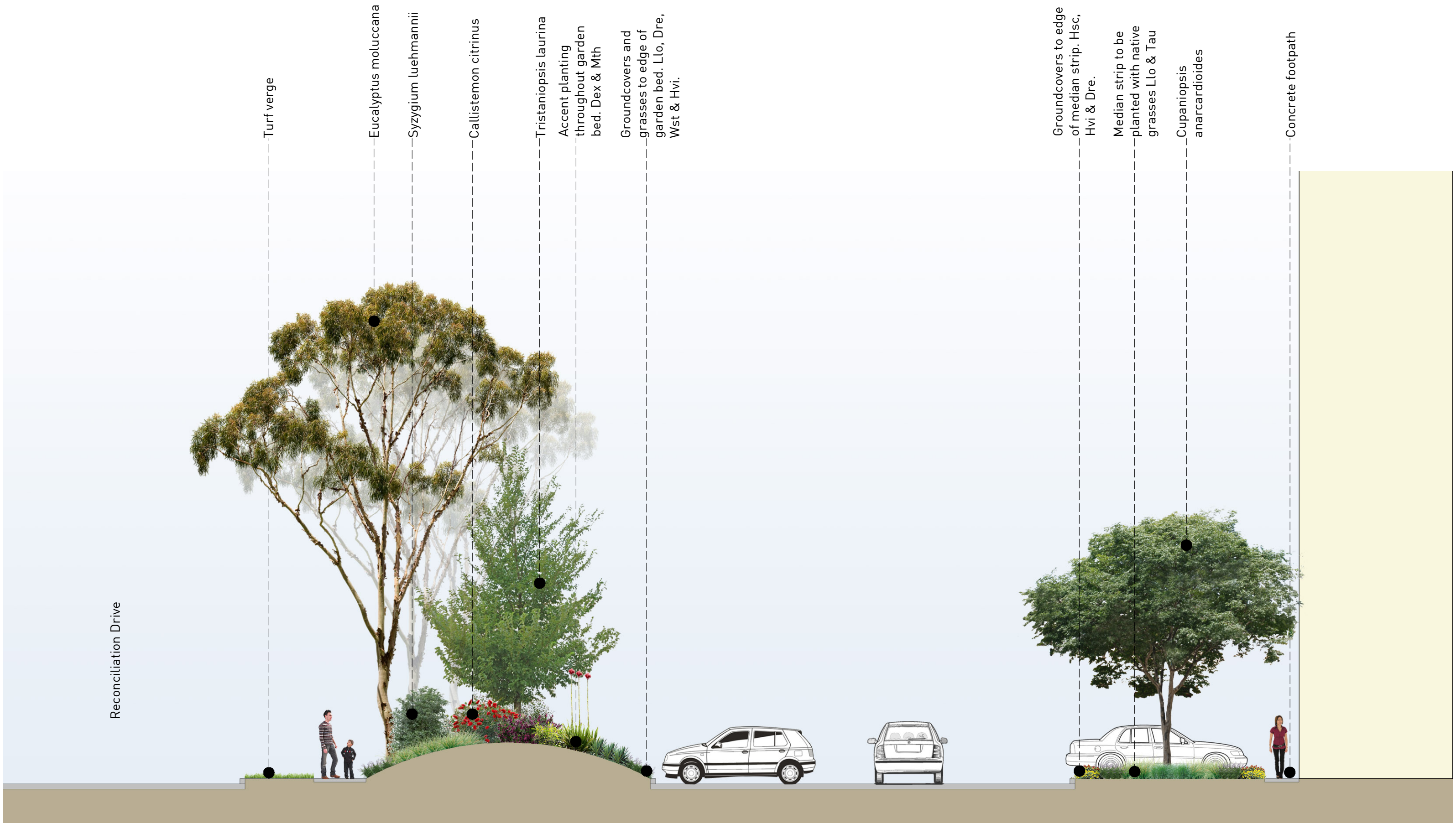
02 Section 2 : Reconciliation Drive L01 1:100 @ A1
