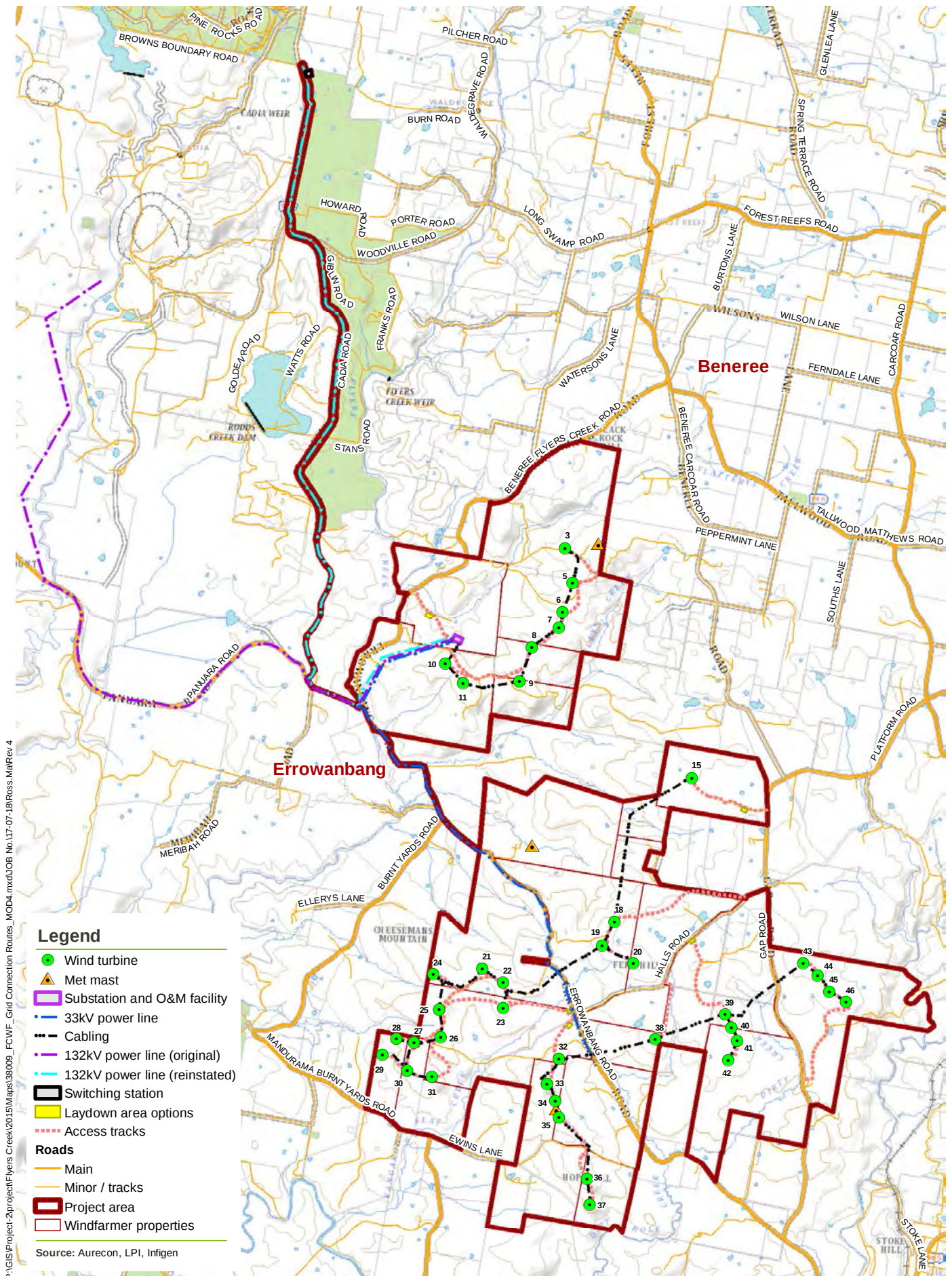
Figure 5: Grid Connection Routes
