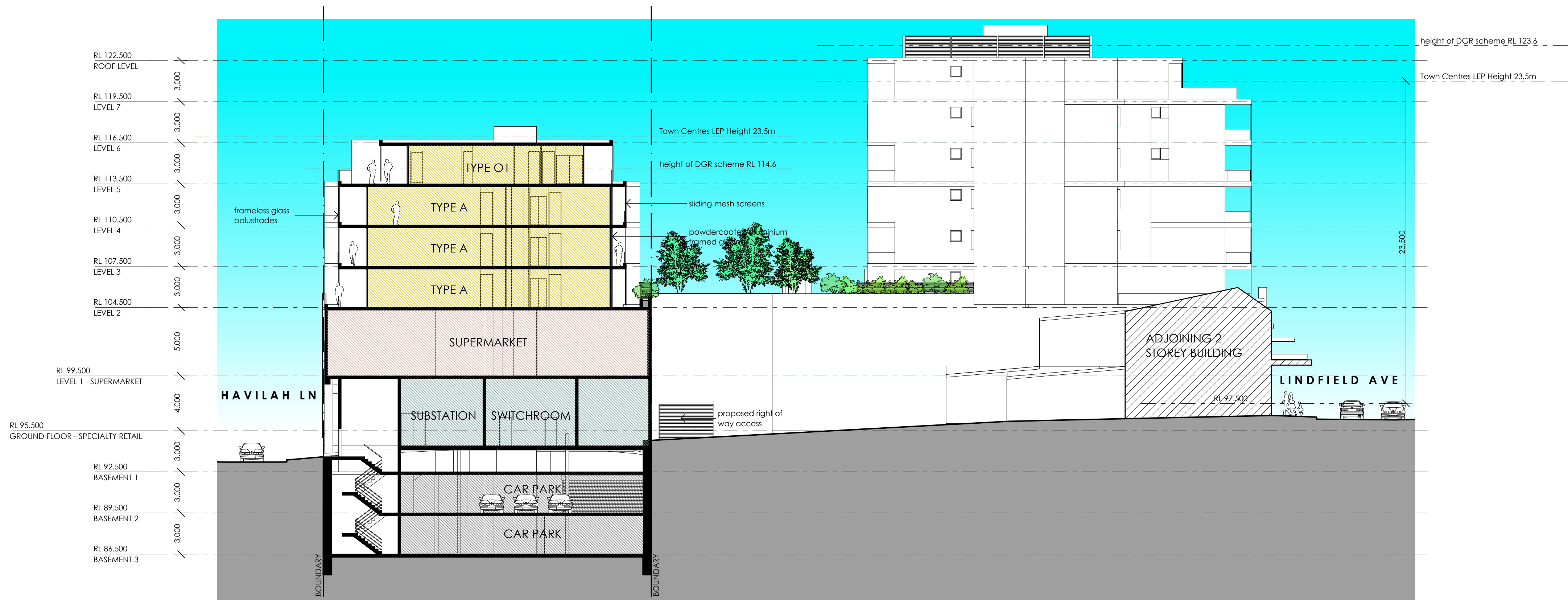
2 SECTION B 1:200
