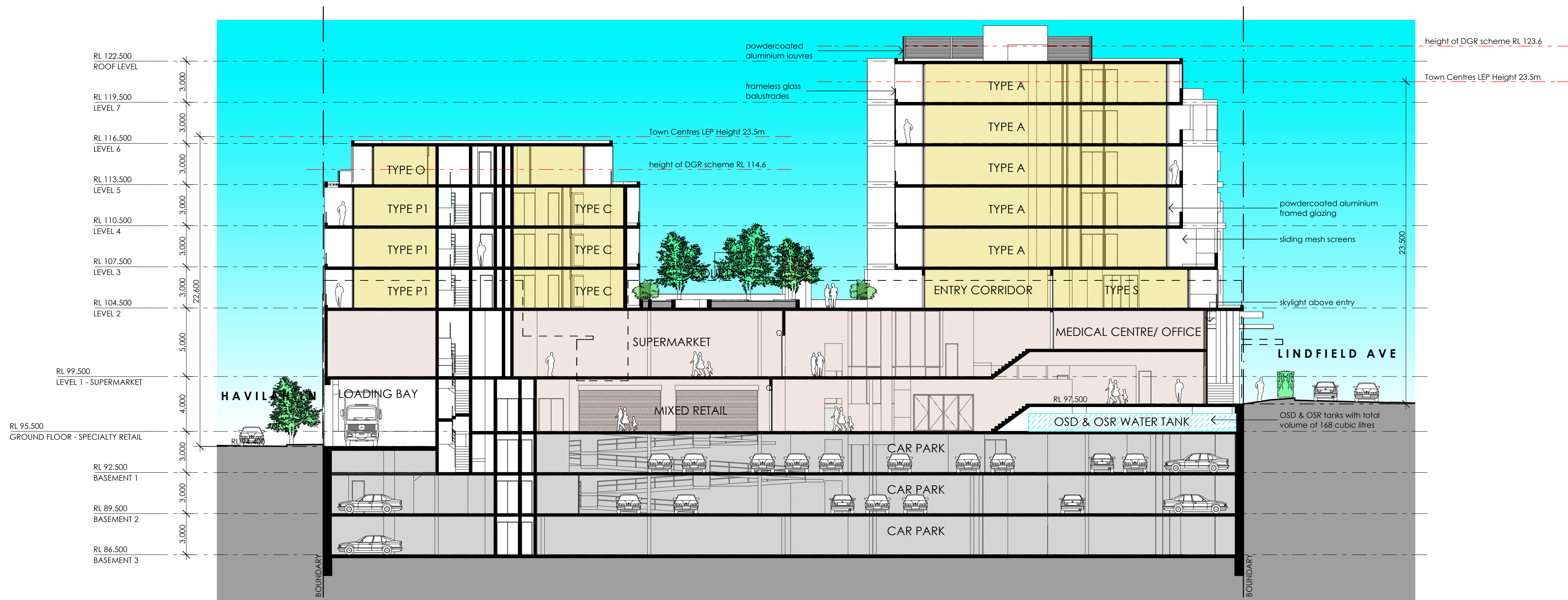
1 SECTION A 1:200
